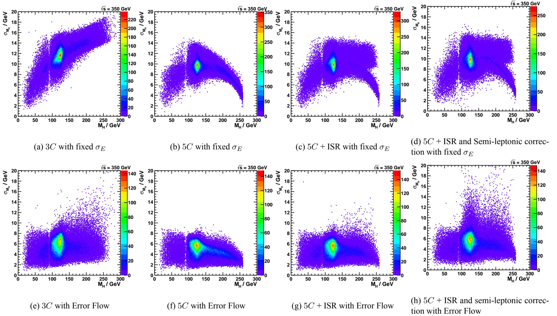
Figure 8.14 – Distributions of the uncertainty on the invariant mass of the Higgs boson as a function of the invariant mass for various fit hypothesis using fixed and jet-specific energy uncertainty.
