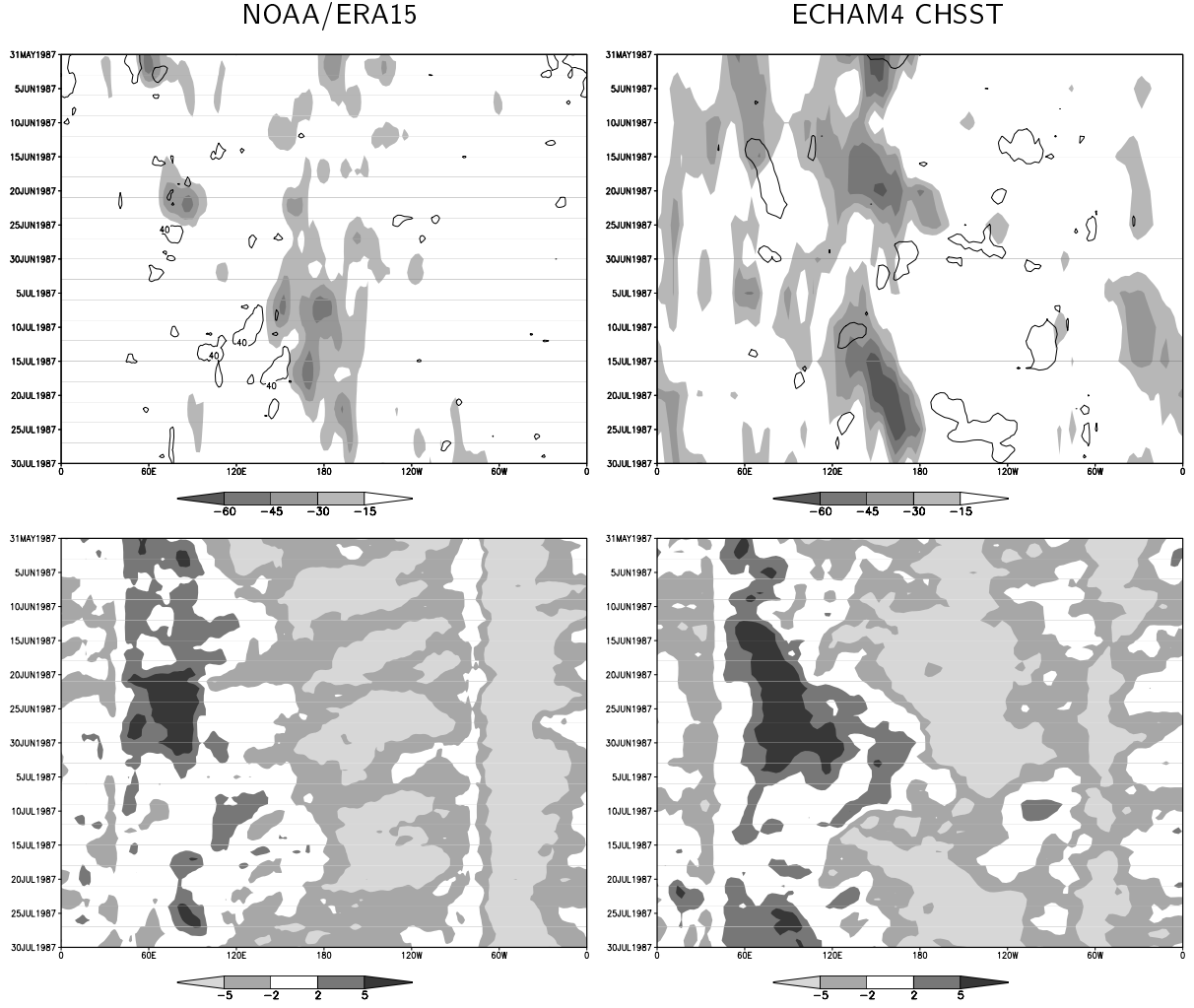
Figure 5.20: Top: OLR anomaly [ W m^{-2} ] (shaded) and the 40 W m^{-2} isoline of latent heat flux anomaly. Bottom: 850 hPa zonal wind [ m s^{-1} ]. All data are averaged between 10°N and 10°S. Left: NOAA OLR and ERA15 latent heat flux and zonal wind, right: ECHAM4 CHSST data.
