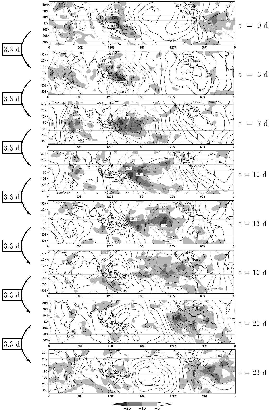
Figure 5.8: Pseudo-Hovmöller diagrams of ECHAM4 NOMARI OLR anomaly [ W \text{ m}^{-2} ] and 200 hPa velocity potential anomaly [ 10^7 \text{ m}^2 \text{ s}^{-1} ]. Negative OLR anomaly (shaded) indicates deep convective anomalies and negative velocity potential anomaly (dotted) indicates large-scale divergent flow. Arrows on the left and the scale on the right point out the time step between the panels as derived by the POP analysis.
