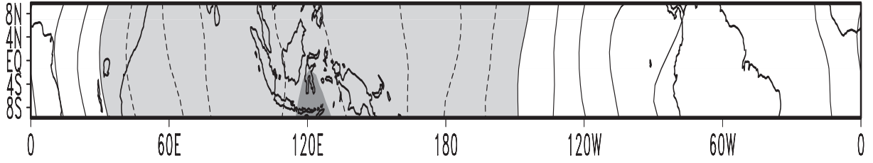
Figure 5.9: ECHAM4 NOMARI first EOF of 200 hPa velocity potential anomaly in the equatorial region. Contour interval is 0.01, negative values are light shaded and the minimum at 120^{\circ}\text{E} is indicated by dark shadings. The EOF pattern explains 33.1% of the total variance.
