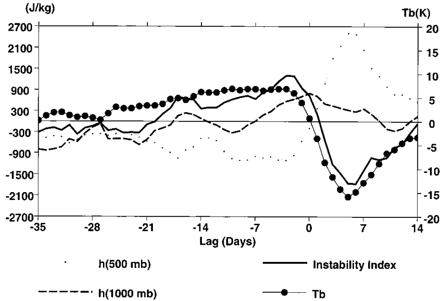
Figure 4.6: Non-maritime continent station composite of moist static energy anomalies ( h ) at 1000 and 500 hPa, instability index h(1000 \text{ hPa}) - h(500 \text{ hPa}) and brightness temperature anomaly ( T_b ), adapted from Kemball-Cook and Weare (2001). Day 0 indicates the onset of convection.
