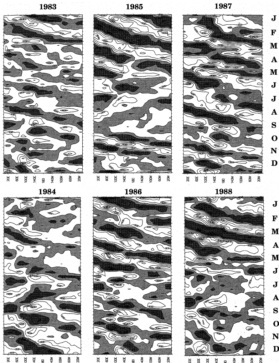
Figure 1.2: Time-longitude diagrams of the 20-100 day filtered velocity potential anomaly at 150 hPa, averaged between 10°N and 10°S, from ECMWF analyses. The contour interval is 2 \times 10^6 \text{ m}^2 \text{ s}^{-1} and negative values are shaded (Slingo et al., 1996).
