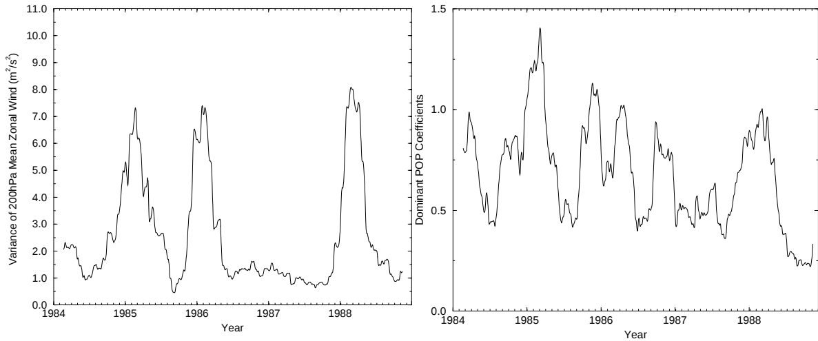
Figure 2.10: ERA15 \overline{u_{200}} -variance averaged between 10^\circ N and 10^\circ S within a 100-day moving window (left) and 100-day running mean of the squared amplitude of the POP coefficients of 200 hPa velocity potential anomalies (right), both reflecting the interannual variability of the IO activity.
