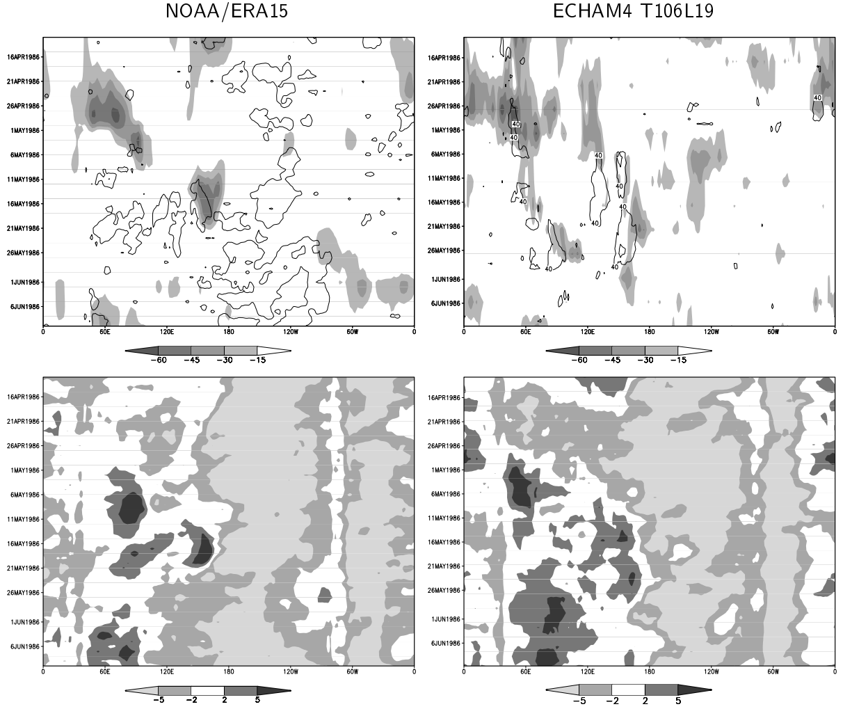
Figure 5.5: Top: OLR anomaly [ W m^{-2} ] (shaded) and the 40 W m^{-2} isoline of latent heat flux anomaly. Bottom: 850 hPa zonal wind [ m s^{-1} ]. All data are averaged between 10°N and 10°S. Left: NOAA OLR and ERA15 latent heat flux and zonal wind, right: ECHAM4 T106L19 data.
