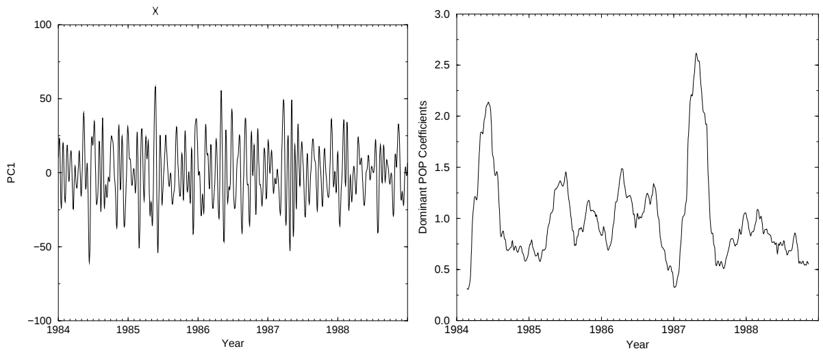
Figure 5.10: Left: ECHAM4 NOMARI PC1, which is used as an index of the activity of the IO. X marks the maximum at the 20th of May 1985 as an identifier for a typical IO. Right: 100-day running mean of the squared amplitude of the POP coefficients of 200 hPa velocity potential anomalies, reflecting the interannual variability of the IO activity.
