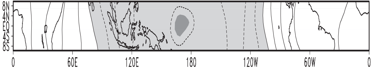
Figure 3.3: ECHAM4 T42L19 first EOF of 200 hPa velocity potential anomaly in the equatorial region. Contour interval is 0.01, negative values are light shaded and the minimum at 170°E is indicated by dark shadings. The EOF pattern explains 34.7% of the total variance.
