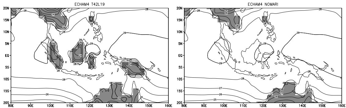
Figure 5.6: Land-sea distribution (land points shaded) and mean surface temperature [ ^\circ\text{C} ] for 1984-1988 of the control experiment (ECHAM4 T42L19, left) and the experiment with the land mass of the maritime continent replaced by sea points (ECHAM4 NOMARI, right).
