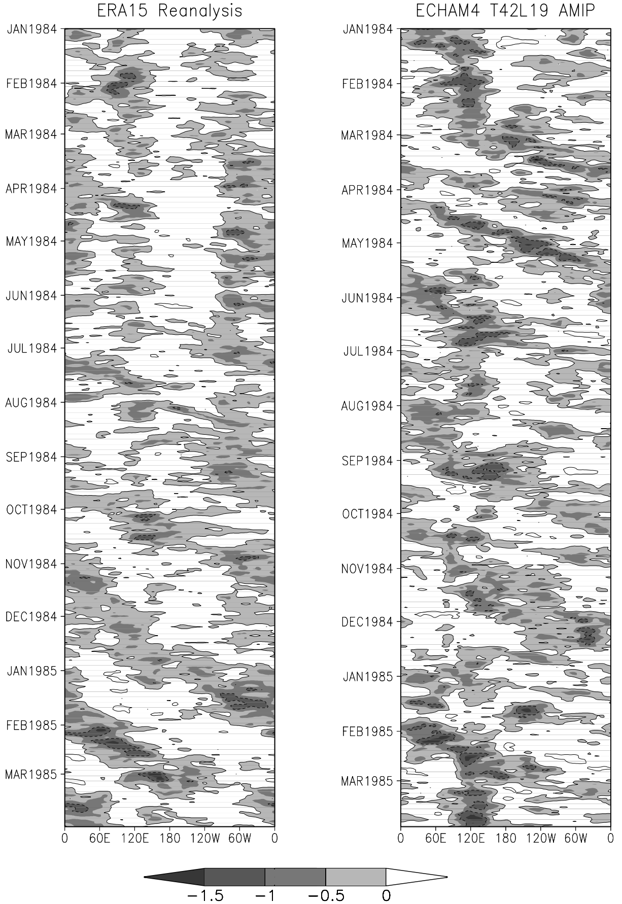
Figure B.1: Hovmöller diagrams of the IO cycle represented by 200 hPa velocity potential anomaly [ 10^7 \text{ m}^2 \text{ s}^{-1} ] averaged between 10^\circ \text{ N} and 10^\circ \text{ S} . Shown is the period from January 1984 to March 1985 for the ERA15 reanalysis and selected GCM experiments. Negative values are shaded.
