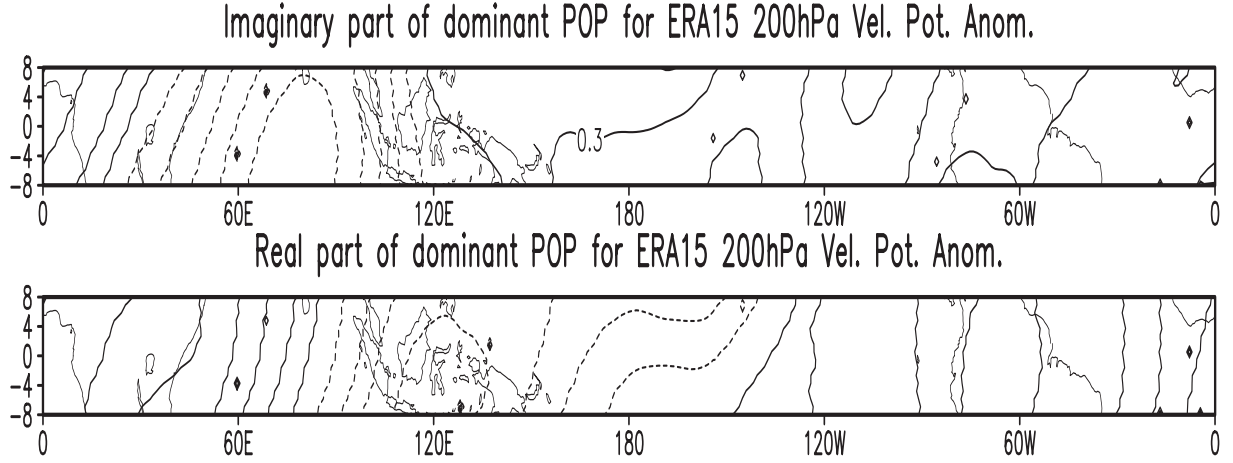
Figure C.2: Imaginary (top) and real (bottom) part of the dominant POP of 200 hPa velocity potential anomalies. Contour interval is 0.3, negative values are dashed and the pattern explains 23.8% of the total variance.
