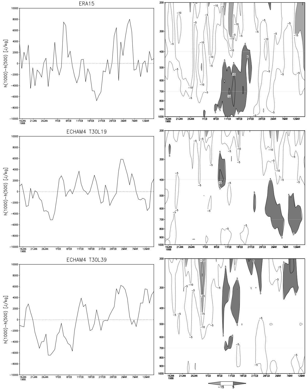
Figure 4.7: Moisture static energy anomalies and the instability index (left) and the vertical profile of the related zonal wind (right) at the equator at 120°E. Top: ERA15, middle: ECHAM4 T30L19, bottom: ECHAM4 T30L39.
