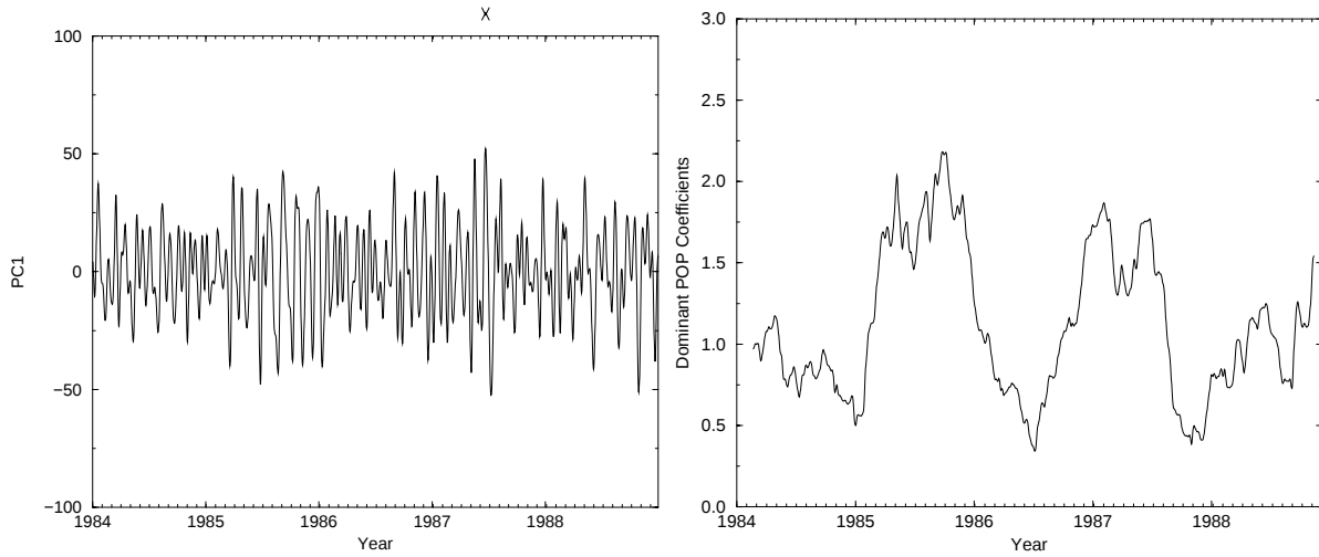
Figure 5.19: Left: ECHAM4 CHSST PC1 which is used as an index of the activity of the IO. X marks the maximum at the 20th of June 1987 as an identifier for a typical IO. Right: 100-day running mean of the squared amplitude of the POP coefficients of 200 hPa velocity potential anomalies, reflecting the interannual variability of the IO activity.
