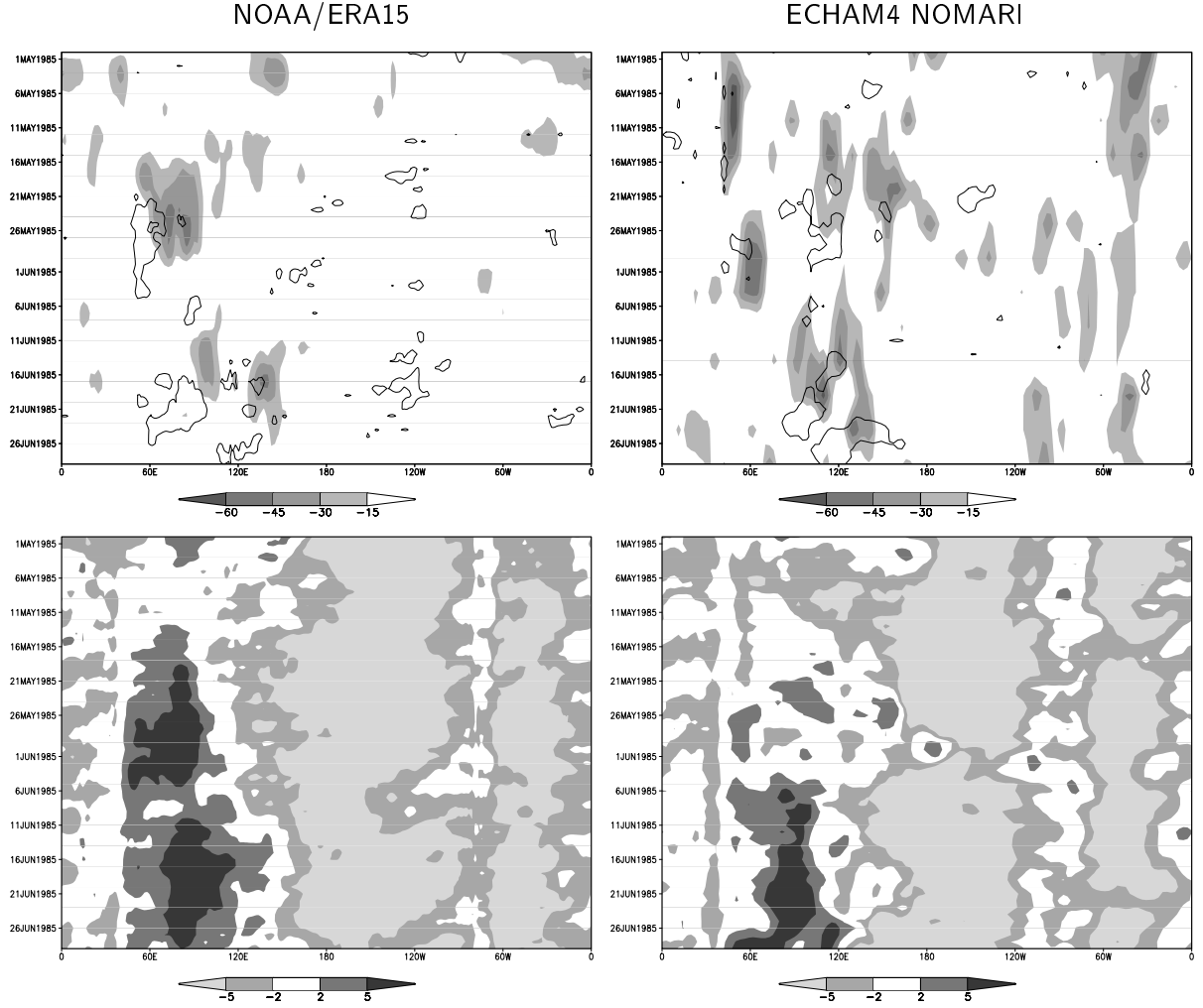
Figure 5.11: Top: OLR anomaly [ W m^{-2} ] (shaded) and the 40 W m^{-2} isoline of latent heat flux anomaly. Bottom: 850 hPa zonal wind [ m s^{-1} ]. All data are averaged between 10^{\circ}N and 10^{\circ}S . Left: NOAA OLR and ERA15 latent heat flux and zonal wind, right: ECHAM4 NOMARI data.
