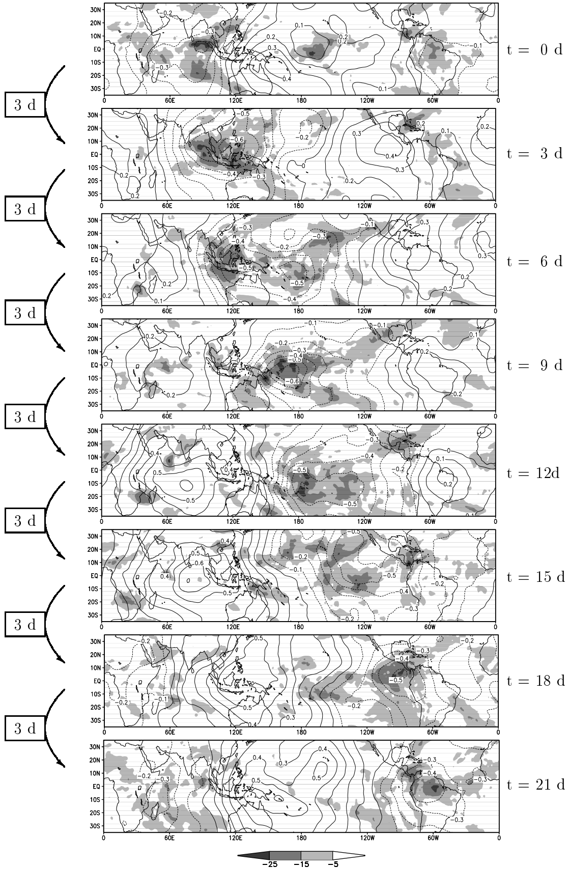
Figure 5.2: Pseudo-Hovmöller diagrams of ECHAM4 T106L19 OLR anomaly [ \text{W m}^{-2} ] and 200 hPa velocity potential anomaly [ 10^7 \text{ m}^2 \text{ s}^{-1} ]. Negative OLR anomaly (shaded) indicates deep convective anomalies and negative velocity potential anomaly (dotted) indicates large scale divergent flow. Arrows on the left and the scale on the right point out the time step between the panels.
