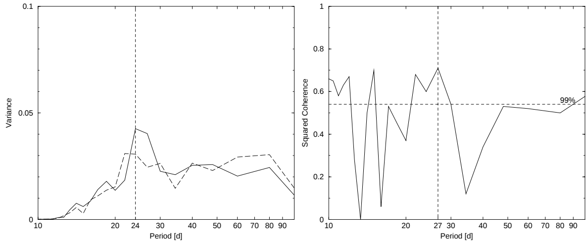
Figure 5.1: ECHAM4 T106L19: spectra of the real (solid line) and imaginary (long dashed line) dominant POP mode (left) and their squared coherence (right). The vertical dashed lines indicate the maxima. The horizontal dashed line depicts the 99% confidence interval of the squared coherence.
