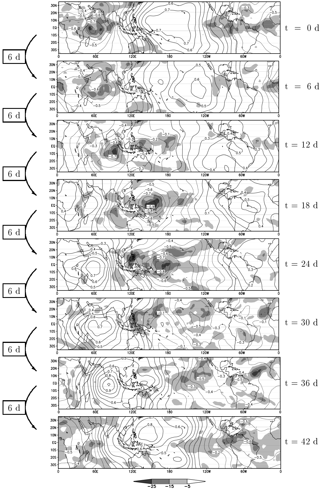
Figure 5.17: Pseudo-Hovmöller diagrams of ECHAM4 CHSST OLR anomaly [ \text{W m}^{-2} ] and 200 hPa velocity potential anomaly [ 10^7 \text{ m}^2 \text{ s}^{-1} ]. Negative OLR anomaly (shaded) indicates deep convective anomalies and negative velocity potential anomaly (dotted) indicates large-scale divergent flow. Arrows on the left and the scale on the right point out the time step between the panels as derived by the POP analysis.
