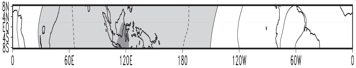
Figure 5.3: ECHAM4 T106L19 first EOF of 200 hPa velocity potential anomaly in the equatorial region. Contour interval is 0.005, negative values are light shaded and the minimum at 117°E is indicated by dark shadings. The EOF pattern explains 34.3% of the total variance.
