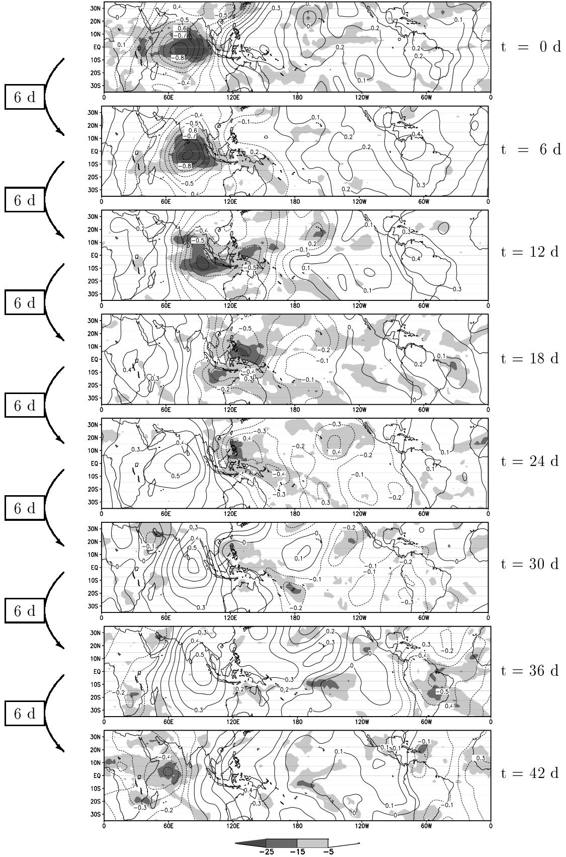
Figure 2.5: Pseudo-Hovmöller diagrams of NOAA OLR anomaly [ \text{W m}^{-2} ] and ERA15 200 hPa velocity potential anomaly [ 10^7 \text{ m}^2 \text{ s}^{-1} ]. Negative OLR anomaly (shaded) indicates deep convective anomalies, and negative velocity potential anomaly (dotted) indicates large-scale divergent flow. Arrows on the left and the scale on the right point out the time step between the panels as derived by the POP analysis.
