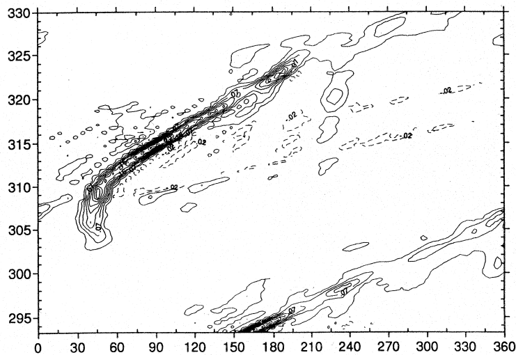
Figure 1.9: Upper-level divergence at latitude 1.6^{\circ}\text{N} simulated with a simplified two-level model. X-axis is longitude in degrees and y-axis is time in days. The contour interval is 3 \times 10^{-6} \text{ s}^{-1} (zero contour suppressed, first positive contour is 1 \times 10^{-6} \text{ s}^{-1} ) (Bladé and Hartmann, 1993).
