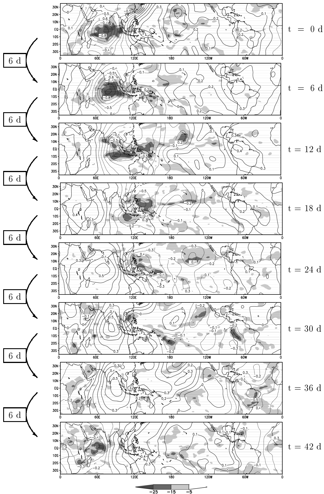
Figure 2.6: As Figure 2.5, but for ERA15 OLR.
