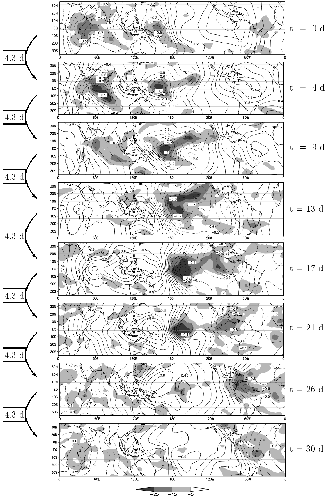
Figure 4.2: Pseudo-Hovmöller diagrams of ECHAM4 T30L39 OLR anomaly [ \text{W m}^{-2} ] and 200 hPa velocity potential anomaly [ 10^7 \text{ m}^2 \text{ s}^{-1} ]. Negative OLR anomaly (shaded) indicates deep convective anomalies and negative velocity potential anomaly (dotted) indicates large scale divergent flow. Arrows on the left and the scale on the right point out the time step between the panels.
