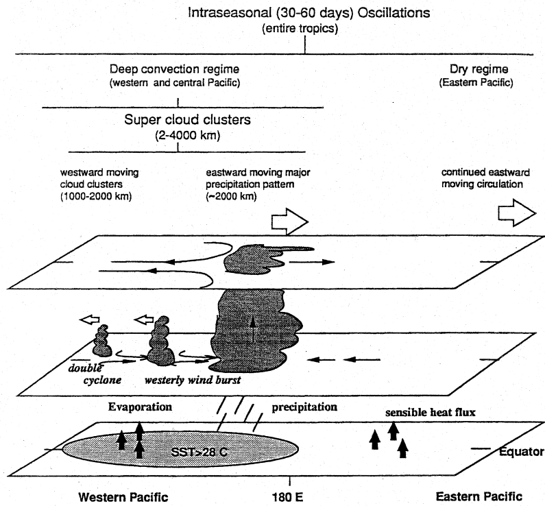
Figure 1.7: Diagram of the hierarchy structure of the IO over the tropical Pacific. Horizontal scales shown are only approximate. Large overlap may occur within the super cloud cluster substructures (Lau et al., 1989).
