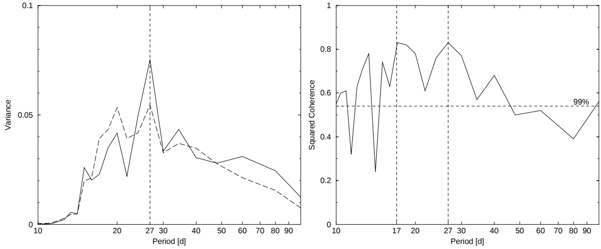
Figure 5.7: ECHAM4 NOMARI : spectra of the real (solid line) and imaginary (long dashed line) dominant POP coefficients (left) and their squared coherence (right). The vertical dashed lines indicate the maxima. The horizontal dashed line depicts the 99% confidence interval of the squared coherence.
