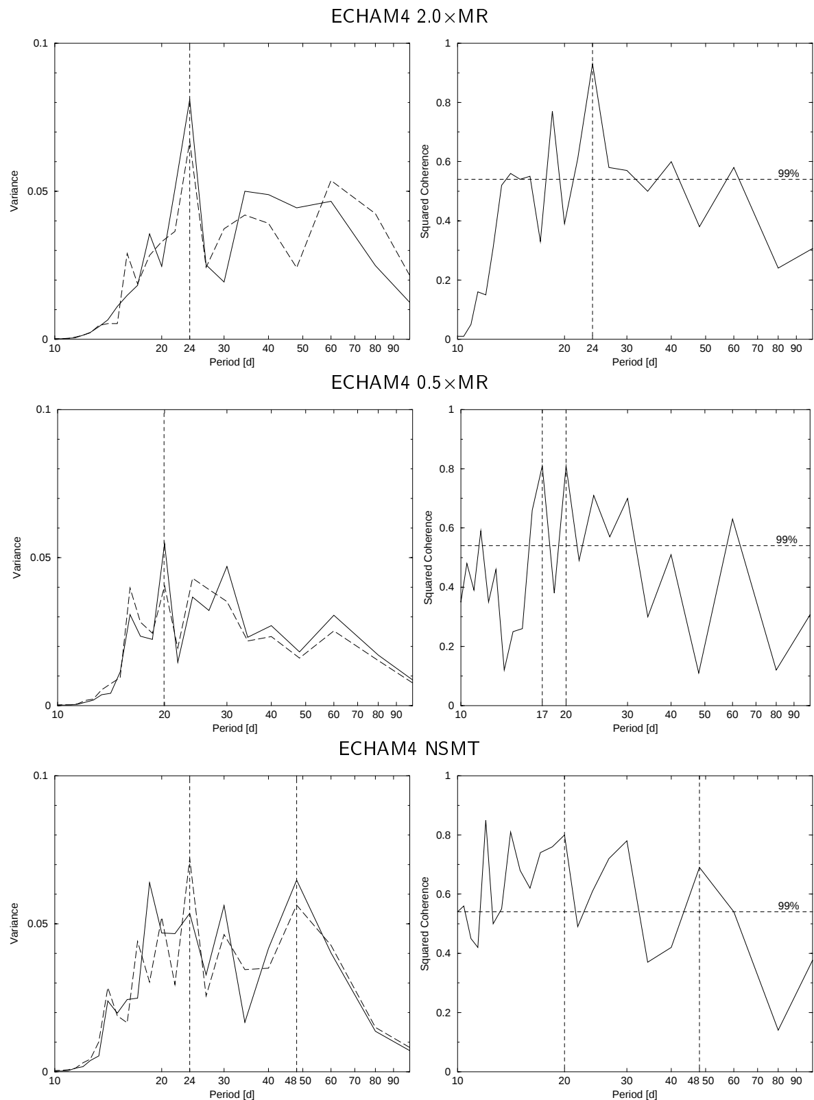
Figure 4.8: Spectra of the real (solid line) and imaginary (long dashed line) dominant POP coefficients (left), and their squared coherence (right) for ECHAM4 2.0 \times MR , ECHAM4 0.5 \times MR and ECHAM4 NSMT. The vertical dashed lines indicate the maxima. The horizontal dashed line depicts the 99% confidence interval of the squared coherence.
