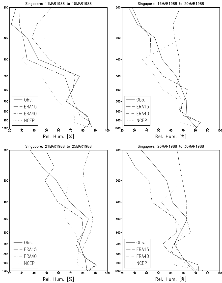
Figure 2.3: Relative humidity during the passage of an IO in March 1988 at Singapore airport ( 1^{\circ}22'N and 10^{\circ}59'E ) for radiosonde measurements (solid), ERA15 (dashed), ERA40 (dash-dotted) and NCEP (dotted).
