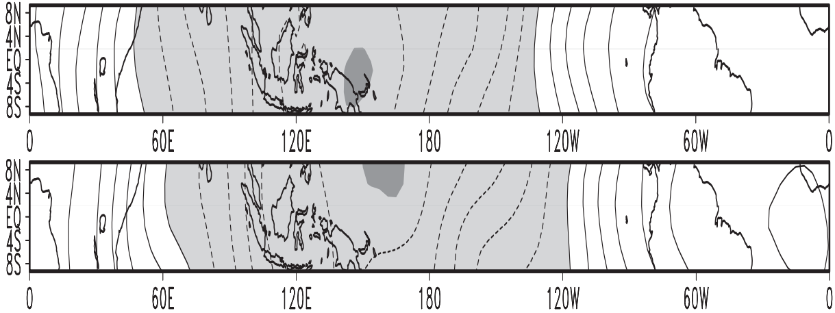
Figure 4.3: ECHAM4 T30L19 (top) and ECHAM4 T30L39 (bottom) first EOF of 200 hPa velocity potential anomaly in the equatorial region. Contour interval is 0.01, negative values are light shaded and the minima at 148^{\circ}\text{E} and 165^{\circ}\text{E} are indicated by dark shadings. The EOF pattern explain 35.2% of the total variance for ECHAM4 T30L19 and 34.6% for ECHAM4 T30L39.
