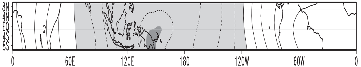
Figure 3.9: ECHAM4/OPYC3 first EOF of 200 hPa velocity potential anomaly in the equatorial region. Contour interval is 0.01, negative values are light shaded and the minimum at 145^\circ\text{E} is indicated by dark shadings. The EOF pattern explains 35.6% of the total variance.
