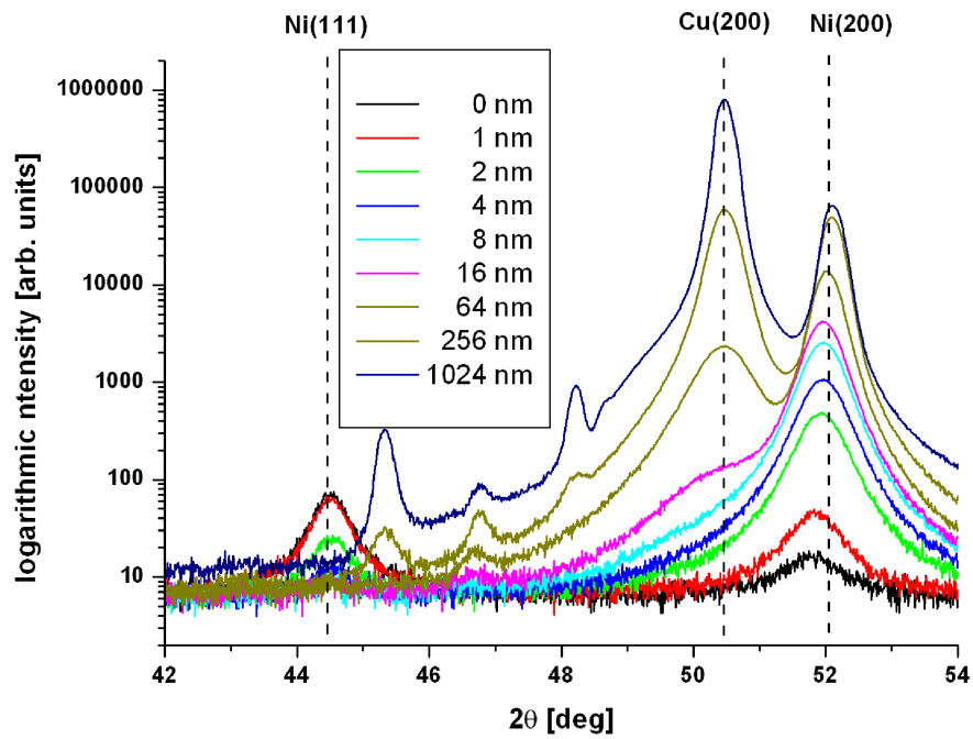
Figure 6.5: Out-of-plane XRD scans as a function of the epitaxial Cu seed layer thickness as given in the legend. A clear switch from polycrystalline growth of Ni to an epitaxial out-of-plane growth of Ni(200) occurs at a Cu seed layer thickness of 4 nm and an increase in the thickness of the seed layer improves the epitaxial quality.
