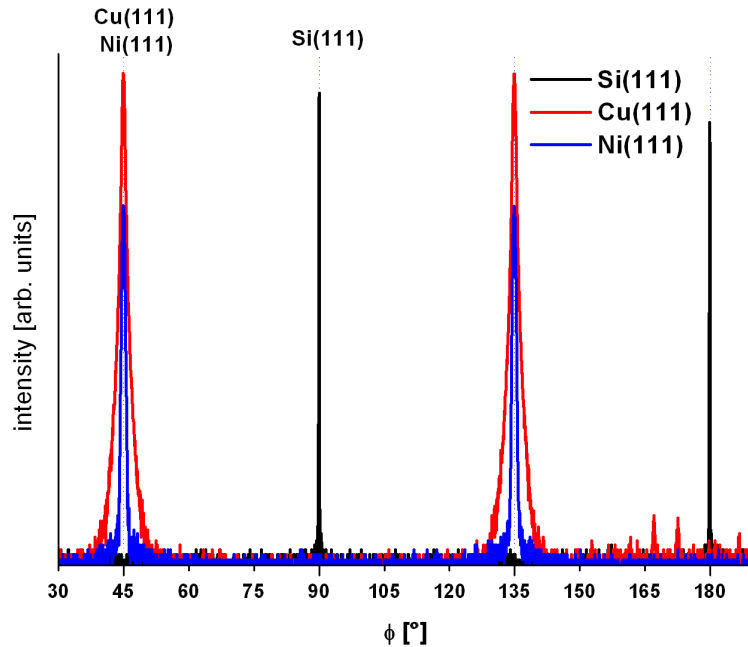
Figure 6.7: The in-plane XRD scans for Si(111), Cu(111) and Ni(111) taken at 54.74° inclination to the (100) plane of the Si substrate. For reasons of clarity only a limited \phi -range is shown. The in-plane orientation of Ni follows that of the Cu seed layer with \Delta\phi = 45^\circ relative to the Si(111) direction.
