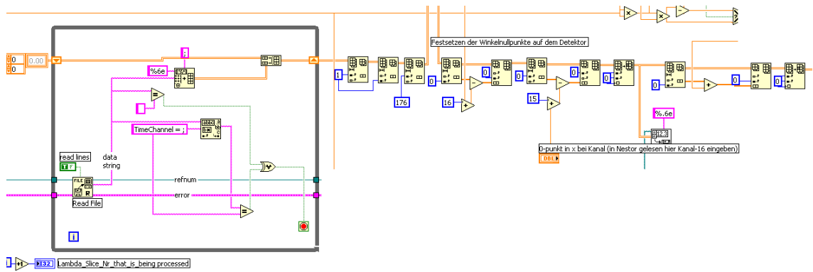
Figure B.20: LabVIEW™ block diagram of the TOF-GISANS evaluation program section "F", which converts the matrices read from the DART input file into arrays of x - y detector channel with corresponding intensities and performs the ballistic correction.
