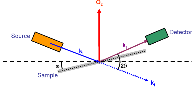
Figure 5.10: Schematic of an \omega - or “rocking” scan: at a fixed 2\theta -angle between the x-ray source and the detector the sample is inclined around the \omega axis. Off-specular intensities in Q_x can thus be probed.
