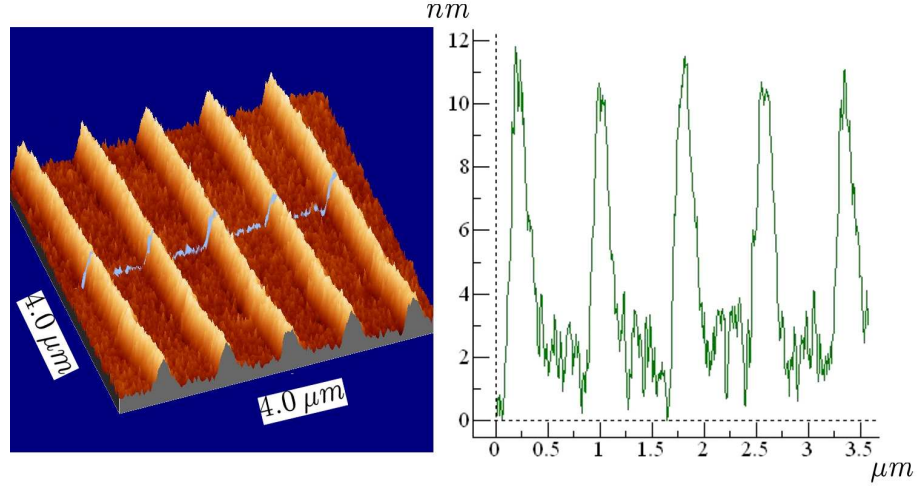
Figure 8.25: 3D representation of the AFM micrograph showing the prepared Ni nanowire sample as obtained from the first pass of the MFM measurements. The scan range is 4\mu\text{m} \times 4\mu\text{m} and a corresponding height trace along the drawn line is shown on the right of the 3D representation.
