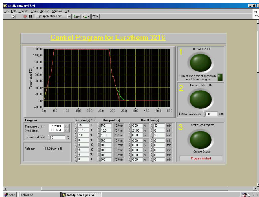
Figure 4.2: LabVIEW™ control program for operation of the CARBOLITE™ HTF 1700 furnace. This allows a temperature sequence to be programmed and recorded to a file.
