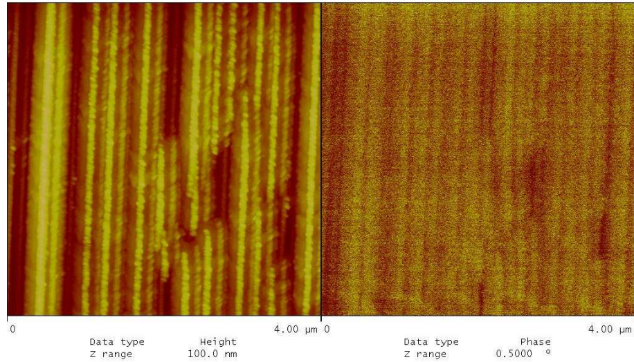
Figure 8.11: AFM and MFM micrographs of the prepared Gd nanowire sample with a scan area of 4\mu\text{m} \times 4\mu\text{m} . The height information overlaps the MFM information making it impossible to extract a reliable MFM signal. The MFM image gives the appearance of probed magnetic stray fields, which is however caused by the topography of the sample.
