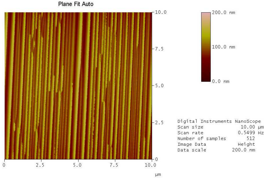
Figure 8.10: AFM micrograph of the prepared Gd nanowire sample with a scan area of 10\mu\text{m} \times 10\mu\text{m} . The height information is clearly dominated by the roughness of the underlying surface and hence only the location of the nanowires could be obtained reliably, not their size.
