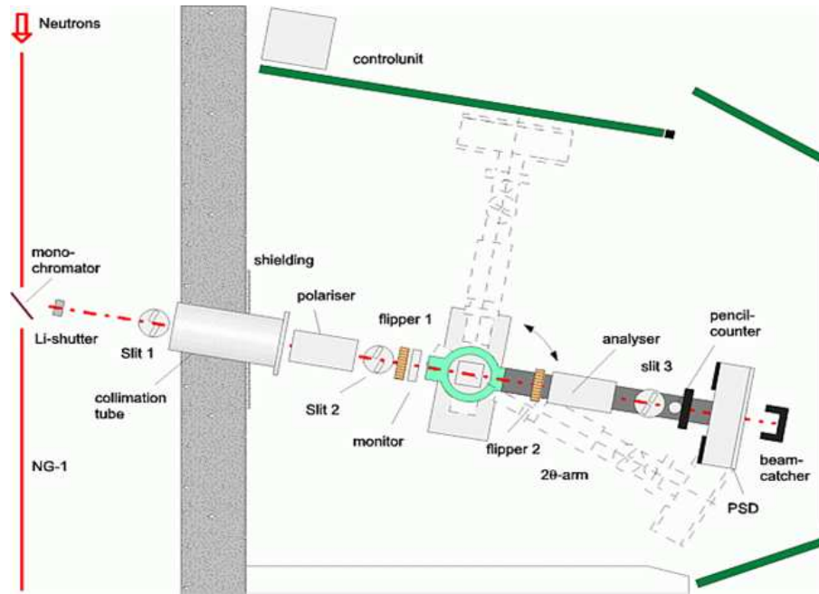
Figure 8.7: Schematic of the NERO reflectometer at the Geestacht Neutron Facility (taken from [102]).
