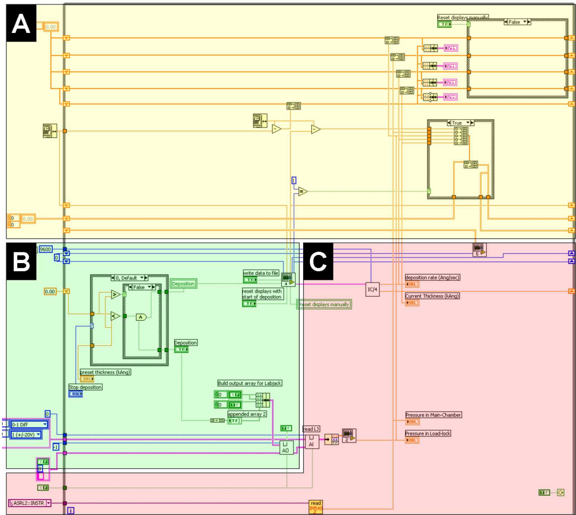
Figure B.9: LabVIEW TM block diagram of the program used to control the deposition process of Ni and Gd nanowires. It contains three functional units: a graph-generation section “A”, a deposition control section “B” and a read-data section “C”.
