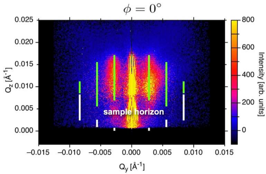
Figure 8.18: Reconstructed integral reciprocal space image for a nominal sample orientation of \phi = 0^\circ with the intensities obtained for all applied wavelengths plotted together with theoretically expected locations of the intensities for reflected (green) and transmitted (white) neutrons. A large portion of the grating truncation rods can be reconstructed allowing for a fast assessment of the lateral structure. In reciprocal space the sample horizon is not at a well defined Q_z value but shifts due to the ballistics before and after the sample.
