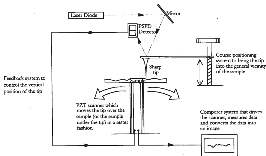
Figure 5.2: Schematic of an AFM/MFM setup (taken from [33].)
