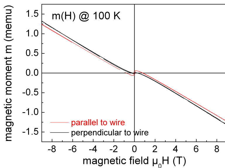
Figure 8.12: Hysteresis loops for Gd nanowires on pre-structured sapphire substrates in the range of -90 kOe to +90 kOe measured at a temperature of 100 K. A strong diamagnetic background from the sample substrate is visible together with a shape anisotropy.
