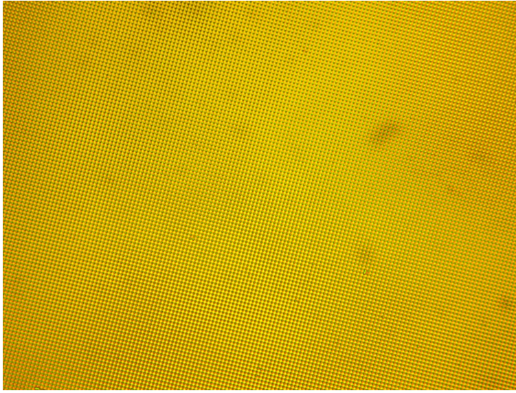
Figure 7.2: Optical micrograph of the structured photoresist mask after double exposure and chemical development. This sub-micrometre structured dot pattern is transferred into the underlying film by physical etching. The darker regions, mainly visible in the right half of the picture, are due to dust particles on the microscope lenses and are not features of the photoresist mask.
