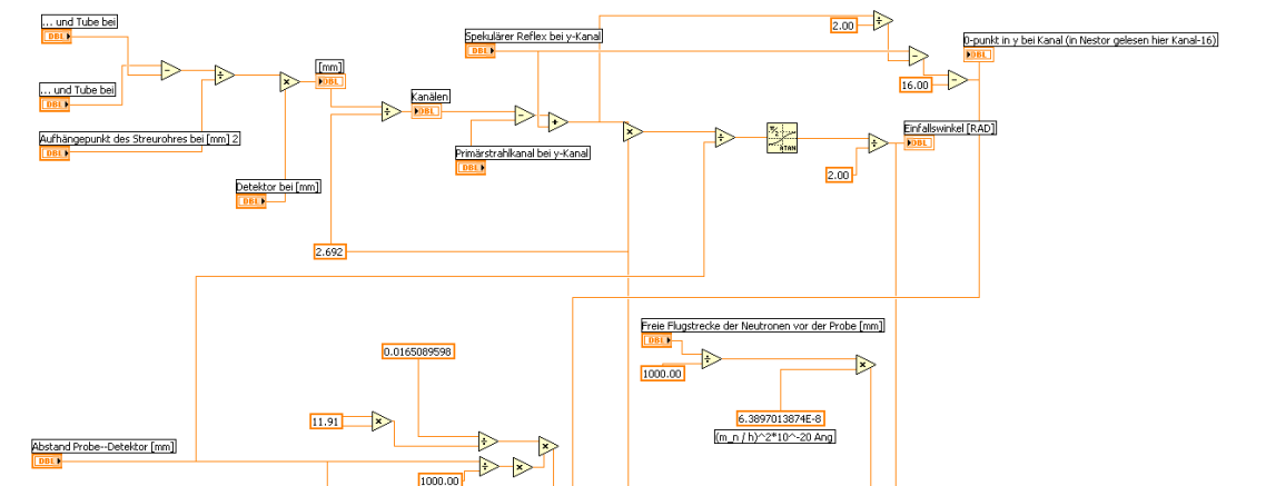
Figure B.16: LabVIEW TM block diagram of the TOF-GISANS evaluation program section “B” which calculates the ballistic correction for each wavelength slice.
