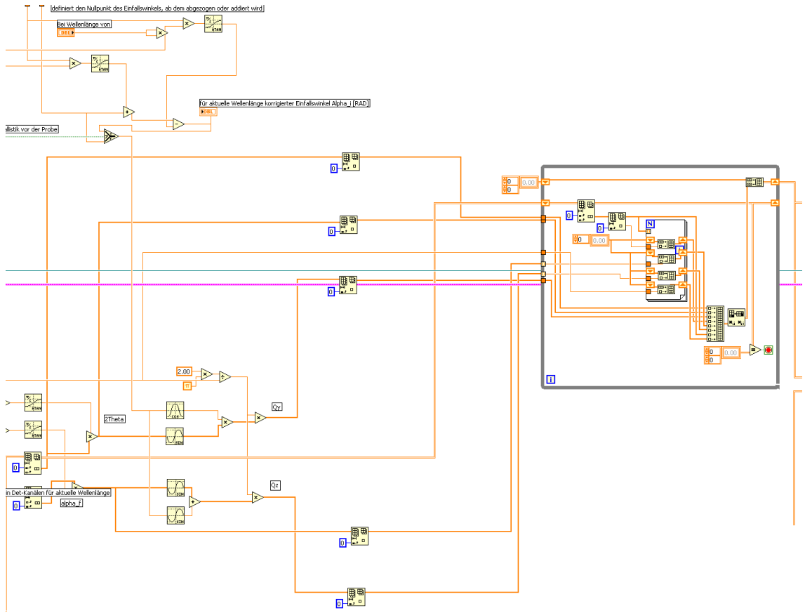
Figure B.18: LabVIEW™ block diagram of the TOF-GISANS evaluation program data-conversion section “D”, which calculates the reciprocal space values.
