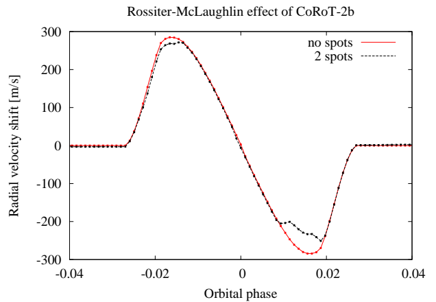
Figure 2.8: Simulation of the Rossiter-McLaughlin effect for CoRoT-2 b. The red curve illustrates the effect if no spots are on the eclipsed section, the black line shows what effect spots have on the shape of the curve. One spot with a size of 0.5 % of the disk is located at 300^\circ longitude, the other one with 0.1 % size is placed at 30^\circ longitude. The planet crosses the disk at stellar phase zero. An asymmetric distribution of starspots shifts the entire RV curve; thus, the black curve was corrected by adding a constant RV value of 35 m/s.
