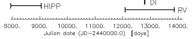
Fig. 1. Time coverage of observations used in this paper. HIPP represents the Hipparcos, DI the Doppler imaging, and RV the radial velocity data sets.
