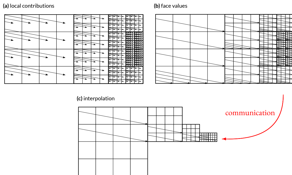
Figure 3.3: The basic steps of the hybrid characteristics method for parallel rays (compare to Rijkhorst et al. (2006) ); a) local contributions as calculated with long characteristics. b) the outgoing face values which have to be communicated. c) example for the interpolation of face values for a particular target cell after the communication step.
