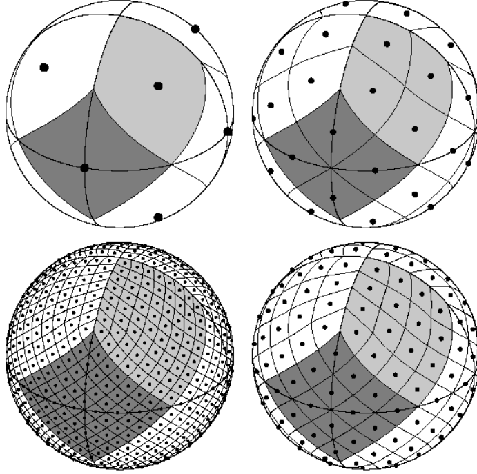
Figure 3.5: The HEALPix tessellation scheme, from Górski et al. (2005). The Area in light grey shows one of the eight (four north, and four south) polar base pixels and the dark grey area shows one of the four equatorial base pixels. Moving clockwise from the upper left panel the base pixels are hierarchically subdivided with the grid resolution parameter equal to N_{\text{side}} = 1, 2, 4, 8 and the total number of pixels N_{\text{pix}} = 12, 48, 192, 768 .
