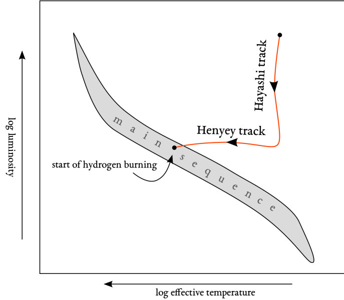
Figure 1.4: Schematics of the Hayashi and Henyey tracks in the Hertzsprung-Russell diagram for a star of one solar mass. The protostar in quasi-hydrostatic equilibrium first appears above the main sequence on the Hayashi track, when the dissociation of H_2 molecules starts. Its luminosity decreases since radiation gets trapped due to the increasing density of the gaseous envelope. After the formation of the second pre-stellar core, the protostar maintains a more or less constant luminosity during the Kelvin-Helmholtz contraction phase (Henyey track) until it reaches the main sequence.
