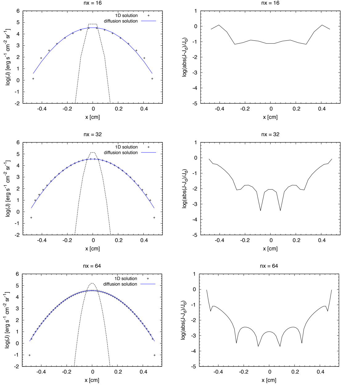
Figure 4.4: Results of the 1D diffusion test for different homogeneous spatial resolutions, top : nx=16 , Mid : nx=32 , bottom : nx=64 . The dashed lines show the initial conditions at t = t_0 determined by the Gaussian solution of the diffusion equation. The initial radiative energy (symbols) is evolved and diffuses outwards until t = 20 \times t_0 is reached and compared to the analytical solution (solid lines) of the homogeneous diffusion equation. For a sufficient spatial resolution, the numerical solution stays within 1% accuracy. At the edge of the domain, the radiation solver deviates from the diffusion solution as radiation leaves the domain while the diffusion solution is valid for an infinite domain.
