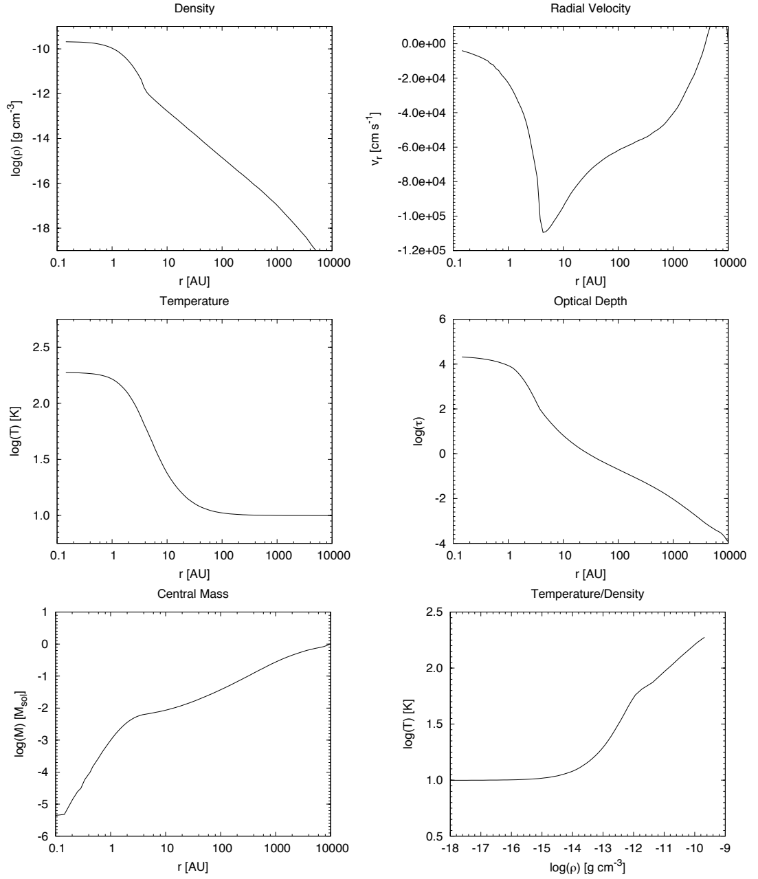
Figure 5.1: Profiles of the collapse simulation after t = 1.036 t_{\text{ff}} ; the maximum density at the core center is \rho_c \approx 2.0 \times 10^{-10} g cm ^{-3} with a temperature of T_c \approx 186 K, a radius of R_{\text{fc}} \approx 4 AU and a mass of M_c \approx 10^{-2} M_{\odot}
