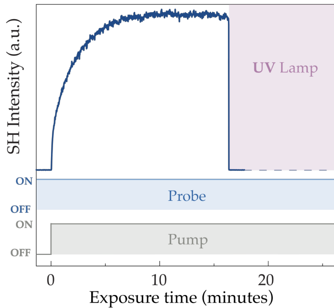
Figure 3.11: Above-bandgap illumination erases the polar state.
