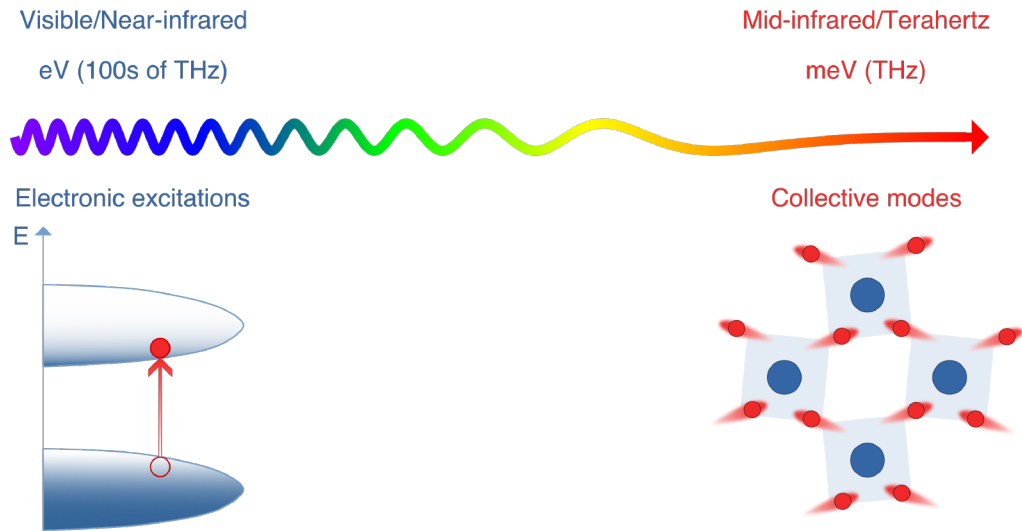
Figure 1.5: Energy scales. Electronic excitations in insulators lie in the electronvolt (eV) energy range. However, collective modes in quantum materials have typical energies of the order of few tens of millielectronvolt (meV). Image adapted from [88].
