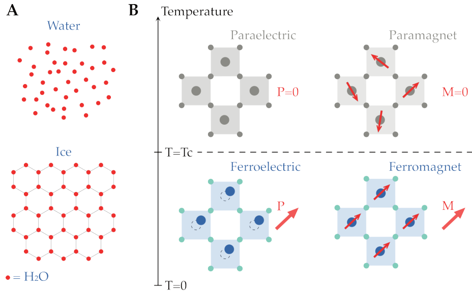
Figure 1.1: Spontaneous symmetry breaking. (A) Structure of water (top) and ice (bottom). (B) Left panel: Above the critical temperature, the material is paraelectric and possesses a center of inversion. Below T_c , the system undergoes a structural transition and breaks inversion symmetry, resulting in a macroscopic polarization P . Right panel: The spins in a paramagnet are randomly oriented. Below T_c , the spins order in a preferential direction resulting in a macroscopic magnetization M .
