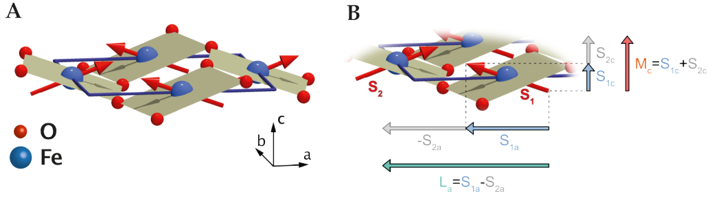
Figure 4.3: Magnetic structure. (A) ErFeO_3 is a canted ferromagnet. Antiferromagnetic order in the ab -plane and small ferromagnetic moment along the c axis. (B) Illustration showing how the ferromagnetic M and antiferromagnetic L vectors can be constructed from the two spin sublattices.
