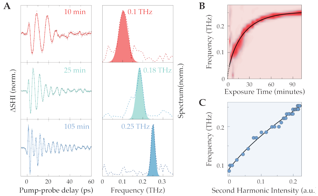
Figure 3.17: Ultrafast Hyper-Raman spectroscopy. (A) Left: mid-infrared-induced modulation of the second harmonic intensity as a function of the pump-probe delay for three representative exposure times. The growing second harmonic offset of Fig. 3.8 was removed. Right: Fourier transform of the time-dependent traces. The red, green and blue peaks are gaussian fits. (B) Fourier transform of the oscillatory traces for different exposure times. The spectra have been normalized for each measurement to better visualize the frequency change and not be affected by the different oscillation amplitudes. The data before minute 5 only contain noise (no second harmonic has grown yet) and, thus, they are not shown. (C) Frequency of the detected oscillations as a function of total second intensity. The dots represent the frequency at which the Fourier spectrum of each time-dependent trace is maximized.
