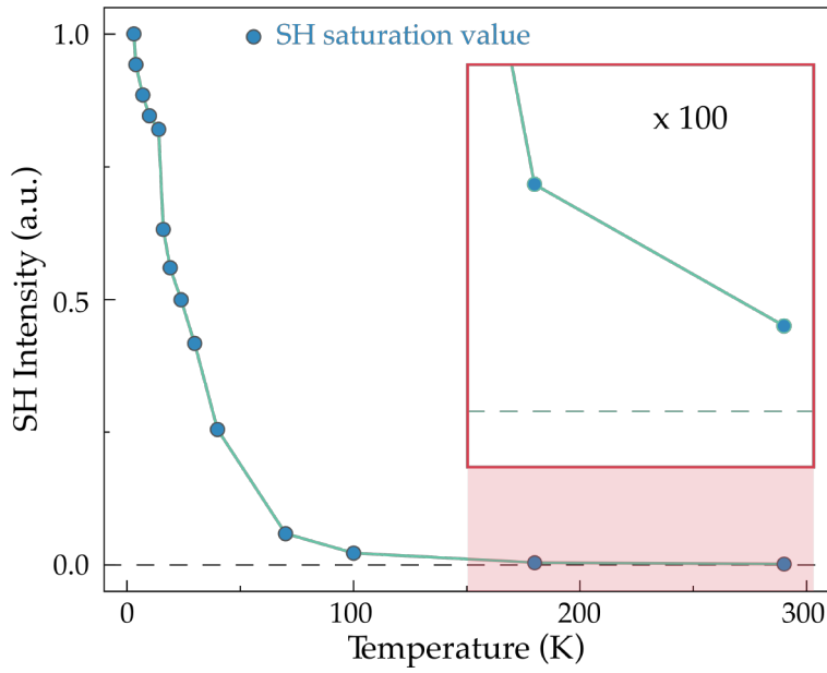
Figure 3.13: Second harmonic temperature dependence. Saturation value of the second harmonic at each temperature (blue dots). All measurements were taken with the same pump wavelength, fluence and pulse duration. Inset: 100 times magnification of the high temperature data.
