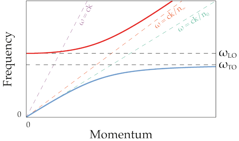
Figure 2.2: Phonon-polariton dispersion. The strong light-matter coupling in the proximity of a phononic resonance results in the formation of hybrid states called phonon-polaritons. Blue: lower polariton branch. Red: upper polariton branch. Between \omega_{TO} and \omega_{LO} there are no available states, i.e. light cannot propagate into the crystal.
