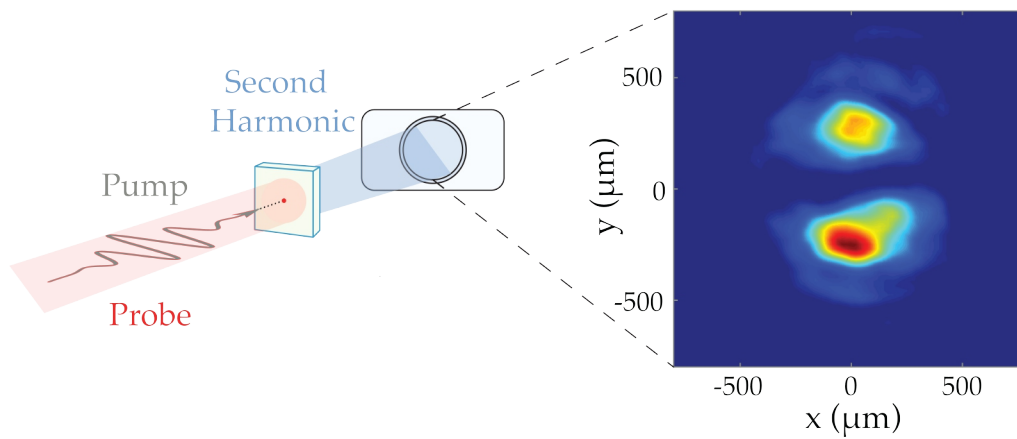
Figure 3.22: Spatial dependence of the second harmonic intensity. Left: Second harmonic shadow imaging setup. Right: second harmonic shadow image.
