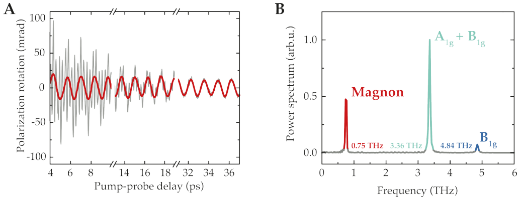
Figure 4.8: Pump-induced dynamics. (A) Polarization rotation as a function of pump–probe delay. The slow, incoherent dynamics has been removed. The oscillations due to coherent phonons (grey) can be filtered out by a low-pass filter (1.5 THz cutoff). The remaining oscillation (red) correspond to the quasi-antiferromagnetic magnon. These measurements were obtained at a pump fluence of 17.6 \frac{\text{mJ}}{\text{cm}^2} . (B) Fourier spectrum of the pump-induced dynamics. Three Raman-active modes can be observed: 0.75 THz, quasi-antiferromagnetic (q-AFM) magnon (red), and 3.36 THz and 4.85 THz, Raman phonons of A_{1g} + B_{1g} (green) and B_{1g} (blue) symmetry, respectively.
