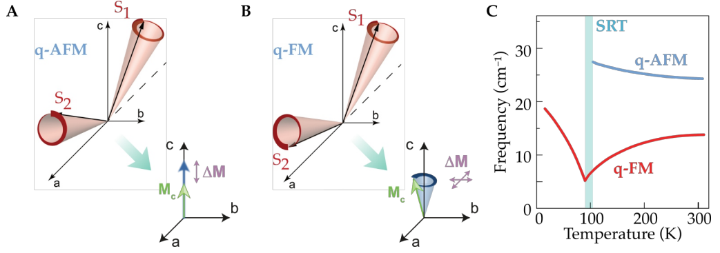
Figure 4.5: Magnon branches. (A) Spin motion associated with the quasi-antiferromagnetic magnon (q-AFM). The magnitude of the ferromagnetic moment M oscillates at the magnon frequency. (B) Quasi-ferromagnetic (q-FM) magnon. The vector M precesses around the c - (above the SRT) or the a - (below the SRT) axis. (C) Magnon frequency as a function of temperature (adapted from [67]).
