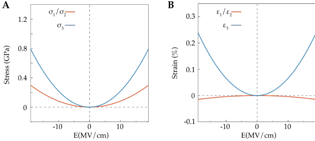
Figure 3.19: (A) First-principles calculations of the phonon-induced stress. (B) Total deformation of the unit cell obtained considering both the phonon-induced stress and the elastic response of the solid.
