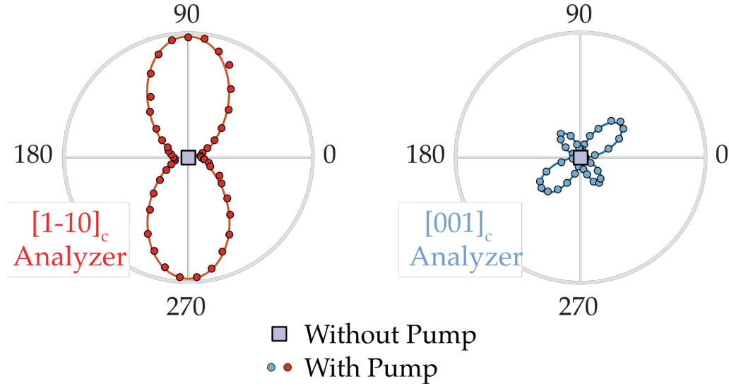
Figure 3.9: Second harmonic polarization dependence. The second harmonic intensity is displayed as a function of the polarization angle of the impinging 2.2 \mu\text{m} probe. Only the second harmonic emitted along the [1 - 10] (left panel) or [001] (right panel) crystallographic directions was measured.
