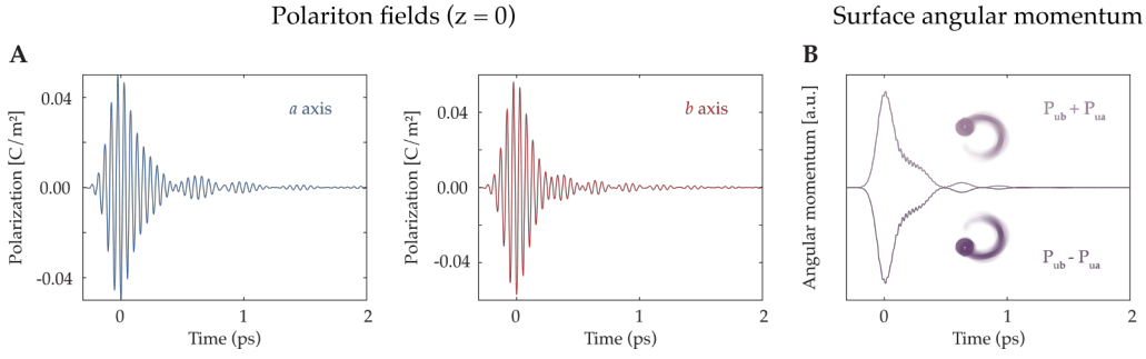
Figure 4.12: Calculated polariton dynamics at the surface. (A) Pump-driven polarizations along the a - (blue line) and b -axis (red line). In the simulations, the phonon-polariton response is initiated by a \frac{MV}{cm} amplitude, 19.5 THz central frequency and 130 fs long pump pulse. (B) Calculated angular momentum of the total phonon-polariton field. Even when simultaneously excited, the optical phonons respond with different initial phases and oscillate at different frequencies resulting in an elliptical polarization. The rotation direction and, as a consequence, the sign of the effective field can be controlled by the initial phase of the infrared-active phonons (light and dark purple).
