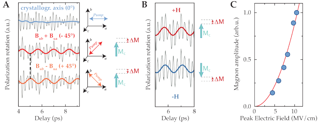
Figure 4.9: (A) Induced dynamics for different pump polarizations (grey). The color lines highlight the magnon oscillations (when present). Blue: while the pump polarization is aligned along one crystallographic axis, no magnon oscillation was detected. Red: when the two orthogonal phonons were excited with the same initial phase ( B_{ub} + B_{ua} ) both Raman phonons and magnon oscillations were observed. Orange: when the two vibrational modes were driven with opposite phases ( B_{ub} - B_{ua} ) the magnon phase changed sign. (B) Magnon dependence on an external magnetic field. The initial orientation of the spins did not affect the magnon phase. (C) magnon amplitude as a function of pump field.
