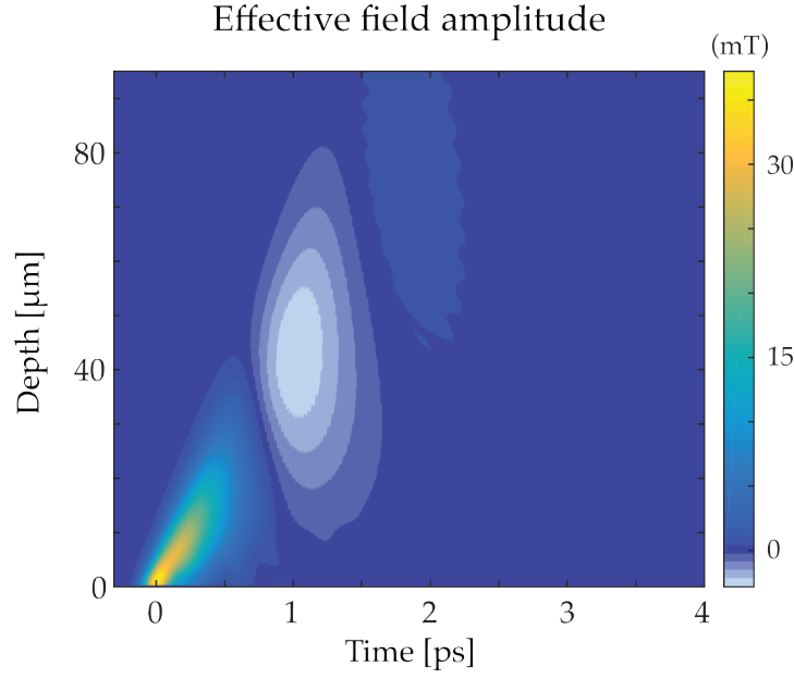
Figure 4.13: Effective field dynamics. The pair of propagating phonon-polaritons generates a time- and space-dependent effective magnetic field. Due to the dephasing of the two modes the rotational motion changes direction at around one picosecond when, however, the phonon amplitude has already decayed significantly.
