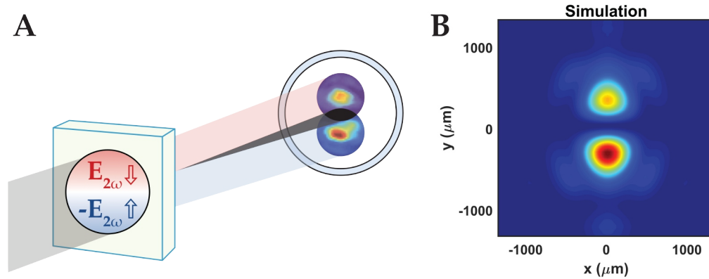
Figure 3.23: Shadow imaging interpretation and simulation. (A) Two antiphase second harmonic fields generated by a bipolar domain structure interfere destructively on the camera. (B) Simulated shadow image.
