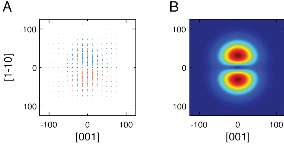
Figure 3.21: Calculated flexoelectric polarizations. (A) polarization vector field in the xy -plane. (B) polarization amplitude in the xy -plane.
