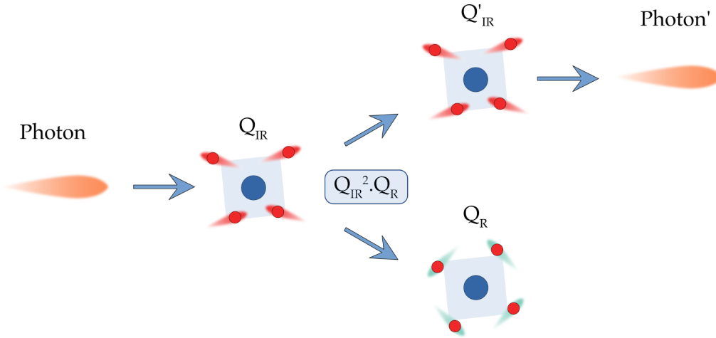
Figure 2.4: Impulsive stimulated Ionic Raman Scattering. A terahertz photon drives coherently an infrared-active phonon. Due to anharmonicities of the crystal lattice, the generated phononic field excites inelastically a Raman phonon. This process also renormalizes the frequency of the infrared-active phonon and of the reemitted terahertz photon. In the figure, the frequency change is indicated by the apostrophe.
