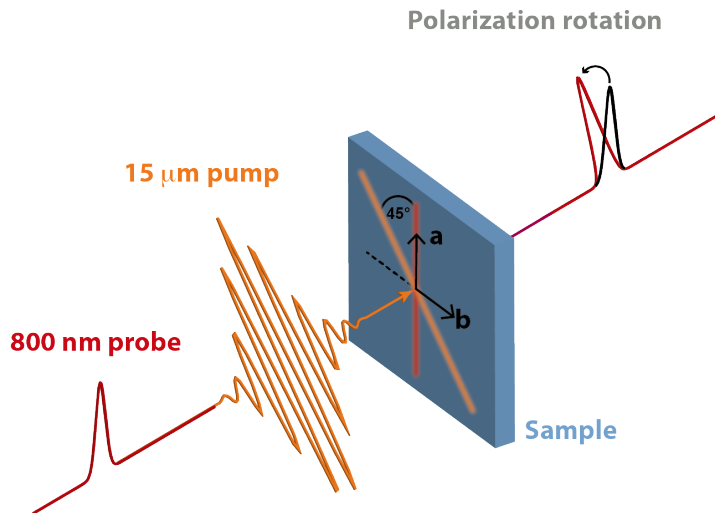
Figure 4.7: Experimental setup. The sample was excited with 20 THz pulses. The induced ultrafast dynamics was probed by looking at the polarization rotation of a linearly-polarized 800 nm-wavelength beam.
