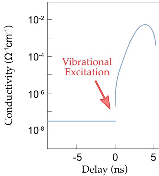
Figure 2.7: Metal-insulator transition in a manganite. Upon vibrational excitation, the conductivity of PCMO changed by several orders of magnitude, confirming the transition to a metallic state (adapted from [103]).
