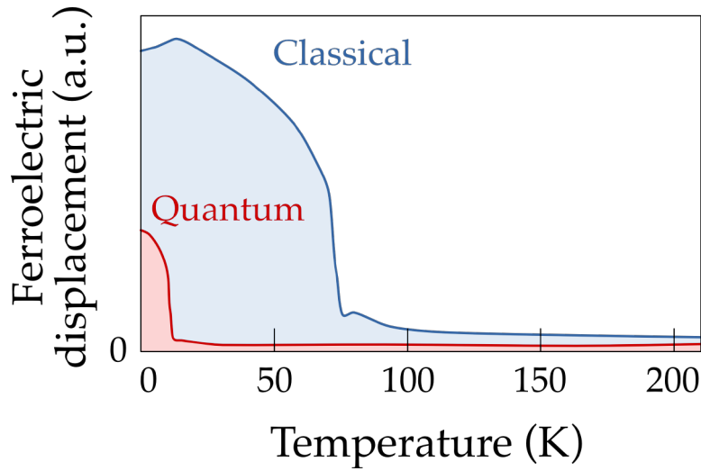
Figure 3.4: Quantum fluctuations suppress the ferroelectric order. The plot displays the size of the ferroelectric displacement in SrTiO_3 as a function of temperature with (red) and without (blue) considering zero-point motion (adapted from [139]).
