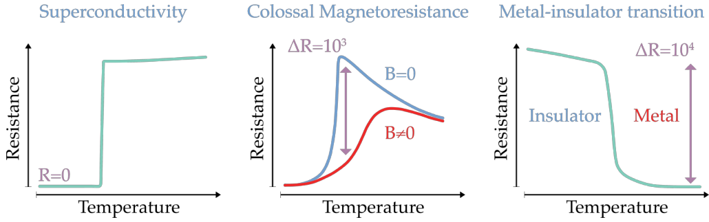
Figure 1.2: Giant collective responses in quantum materials. Left panel: At T_c the resistance of a superconductor becomes identically zero (adapted from [87]). Center panel: In a magnetoresistive material the application of an external magnetic field can change the resistance by several order of magnitude (adapted from [20]). Right panel: In an insulator-to-metal transition a colossal change in resistance occurs at T_c (adapted from [137]).
