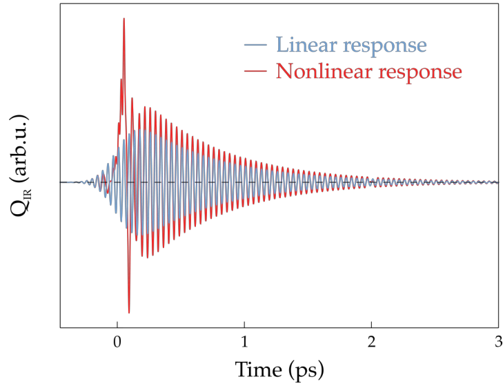
Figure A.2: Comparison between the response of a linear (blue) and a nonlinear (red) oscillator, driven by the same resonant electric field pulse.
