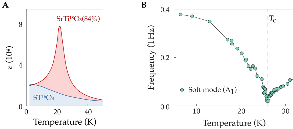
Figure 3.5: Induced ferroelectricity by isotope substitution. (A) dielectric function as a function of temperature in unsubstituted, paraelectric (blue) and in 84% isotope-substituted, ferroelectric (red) \text{SrTiO}_3 (adapted from [126]). (B) Frequency of the lowest energy (“soft”) phonon in isotope-substituted \text{SrTiO}_3 (adapted from [115]).
