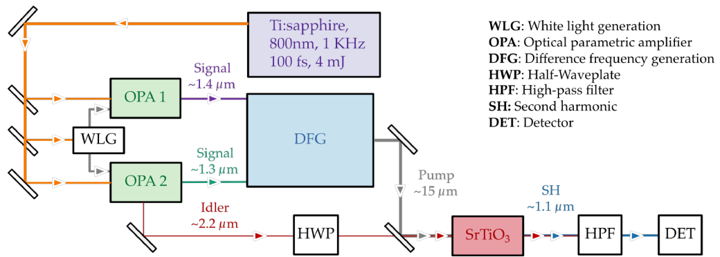
Figure B.1: SrTiO_3 setup.
