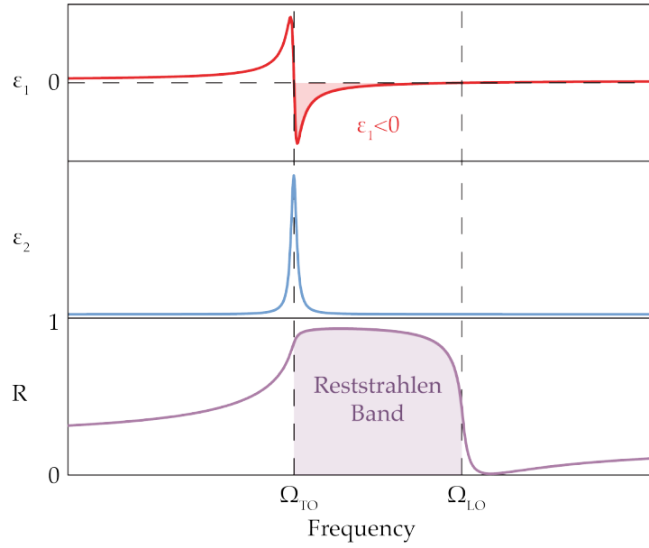
Figure 2.3: Optical properties of an infrared-active phonon in an insulator. Top: real part of the dielectric function. Middle: imaginary part of the dielectric function. Bottom: reflectivity.
