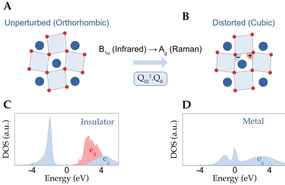
Figure 2.8: Structurally driven electronic transition. (A) Crystal structure of unperturbed PCMO . The materials is orthorhombic. (B) Crystal structure of the dynamically distorted phase. The nonlinear coupling between the infrared and Raman phonons transiently reduces the octahedra rotations, resulting in a more cubic structure. (C) Electronic density of states in the orthorhombic phase. The material is an insulator. (D) Density of states in the cubic phase. Following a phonon-driven collapse of the gap, the material became a metal. The image is adapted from [113].
