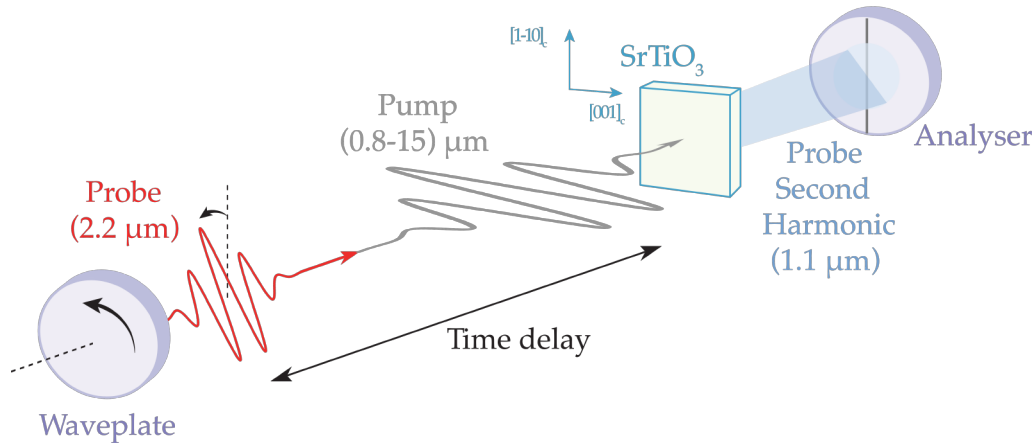
Figure 3.7: Experimental setup. The sample (green) was excited with tunable pump pulses (0.8 to 15 \mu\text{m} , gray line) impinging at normal incidence. The probe pulse (2.2 \mu\text{m} wavelength, red line) polarization was controlled with a half-waveplate. The generated second harmonic (1.1 \mu\text{m} , blue) was detected in transmission. When needed, orthogonal polarization components of the second harmonic could be isolated by an analyzer, that is, a polarizer. The full width at half maximum (FWHM) spot sizes were 72 \mu\text{m} and 52 \mu\text{m} for the pump and the probe beams, respectively.
