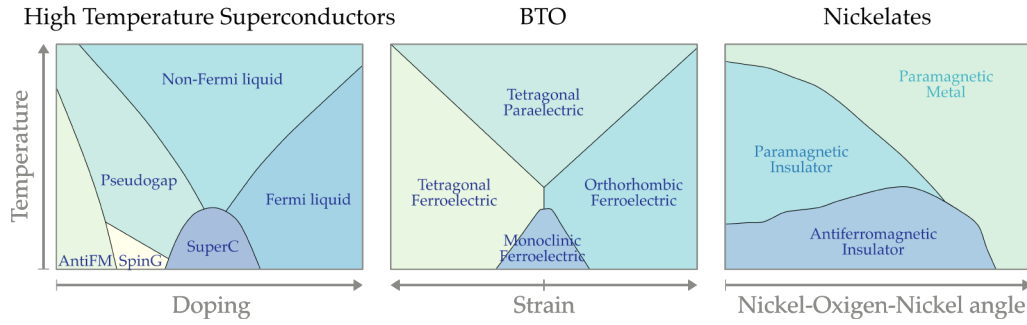
Figure 1.4: Phase diagrams of quantum materials. Left panel: prototypical phase diagram of high-temperature superconductors (adapted from [22]). Center panel: calculated phase diagram of BaTiO_3 as a function epitaxial stress (adapted from [108]). Right panel: phase diagram of rare-earth nickelates ( RNiO_3 ) as a function of Ni-O-Ni angle controlled by changing the rare earth R (adapted from [18]).
