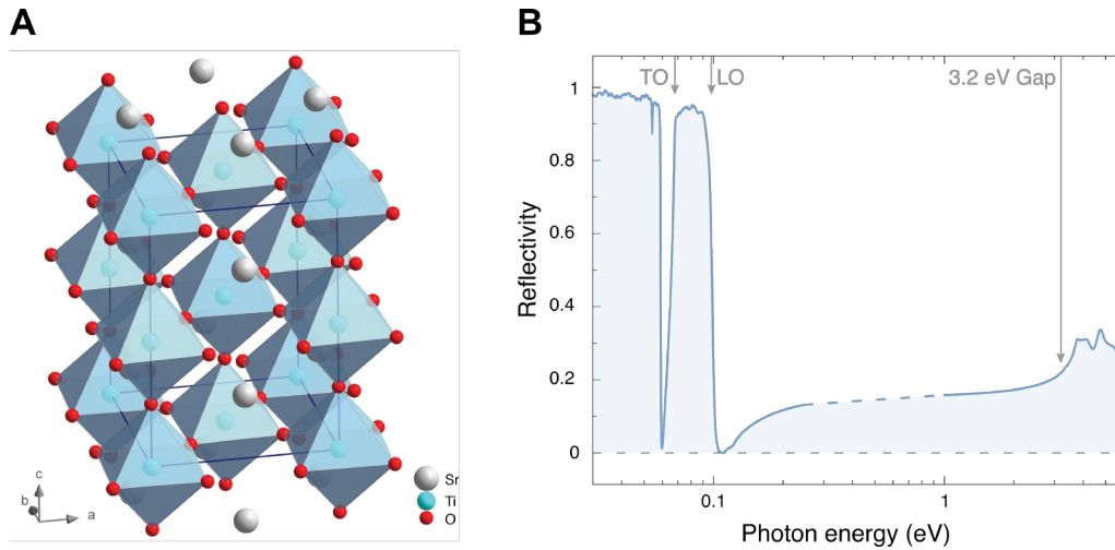
Figure 3.2: (A) low-temperature tetragonal structure of SrTiO_3 (from [60]). (B) Reflectivity. The grey arrows highlight the TO and LO frequency of the highest energy phonon and the position of the optical gap. The data for photon energies smaller than 0.2 eV were measured with an FTIR. The data for photon energies higher than 1 eV were adapted from [23].
