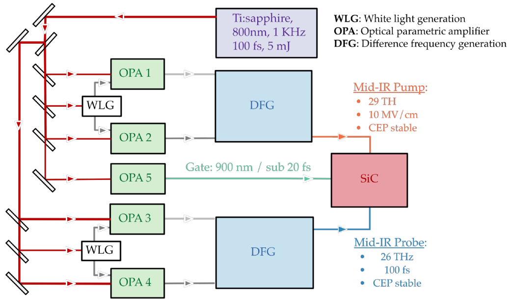
Figure B.3: SiC setup.
