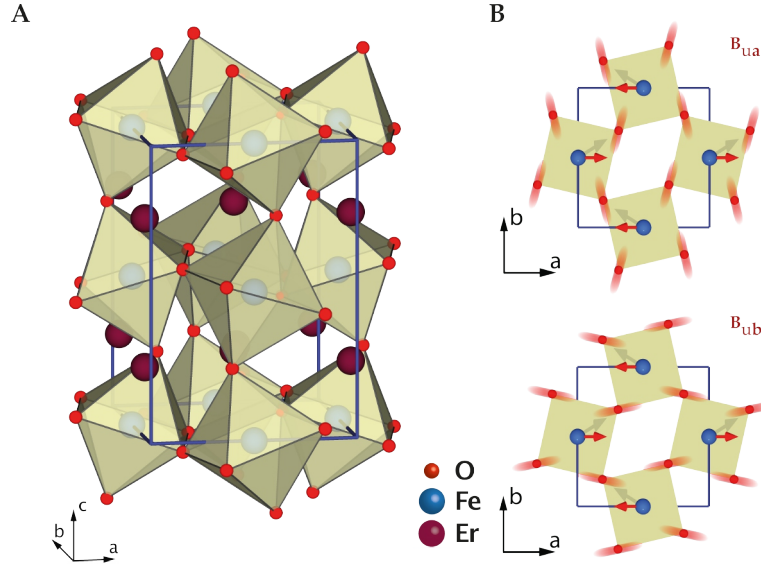
Figure 4.1: (A) Crystal structure of ErFeO_3 . (B) Calculated phonon eigenvectors. The B_{1ua} and the B_{1ub} are polarized along the a and b crystallographic axes, respectively. The highest energy phonons are characterized by the motion of the lighter atoms, oxygen in this case.
