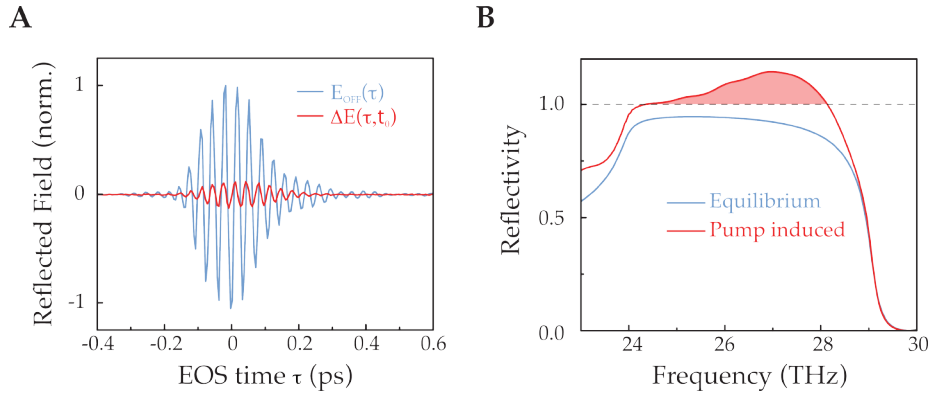
Figure A.5: (A) Electric field reflected from the sample at equilibrium (blue) and simultaneously measured pump-induced change (red). (B) Equilibrium (blue) and nonlinear (red) reflectivity of SiC .
