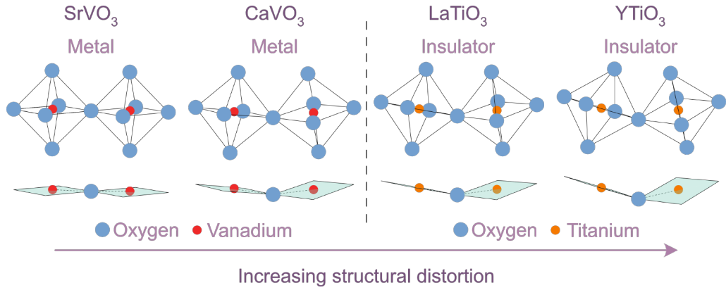
Figure 1.3: Crystal structures of SrVO_3 , CaVO_3 , LaTiO_3 and YTiO_3 . For clarity, part of the unit cell and the Sr , Ca , La and Y ions are not shown. The blue spheres represent the oxygen ( O ) ions while the red and orange spheres represent the transition metal ( TM ) ions. The bottom part highlights the TM - O - TM bond and how it is affected by the deformation. The arrow indicates the direction of increasing structural distortion which also corresponds to a growing electronic localization. The image is adapted from [95].
