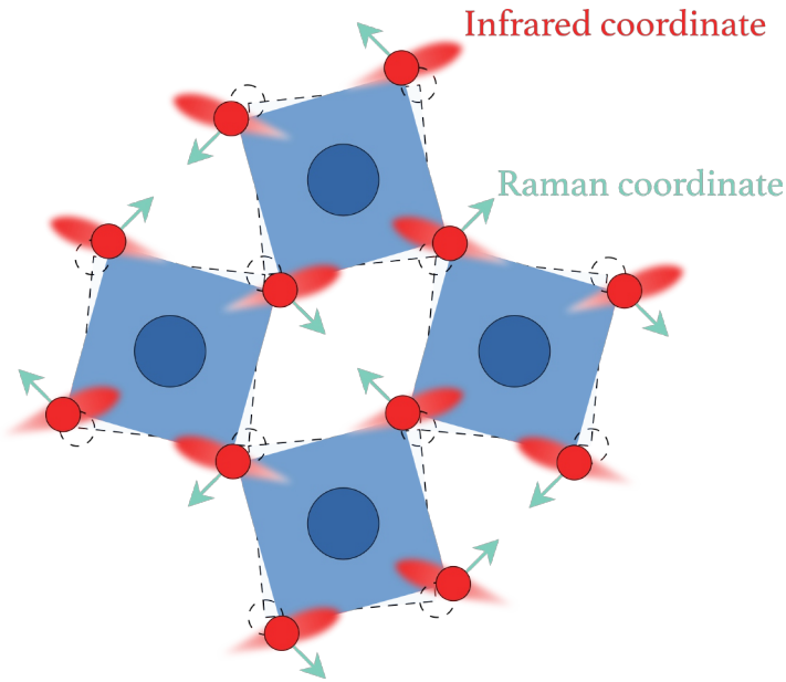
Figure 2.6: A new, transient structure. As long as the driven infrared phonon is oscillating, the ions move along the Raman coordinate to create a new crystal structure.
