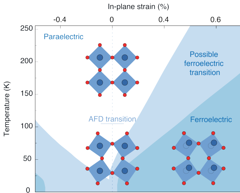
Figure 3.6: Strain-induced ferroelectricity. The phase diagram is obtained by minimizing the total free energy of SrTiO_3 as a function of polarization and strain. The dark blue areas indicate the regions of the diagrams where the material is calculated to be ferroelectric. The light blue areas indicate the range of temperatures and strain values in which the transition could occur. The image is adapted from [73].
