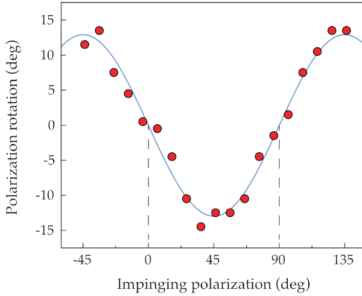
Figure 4.6: Static room-temperature birefringence of ErFeO_3 . A half waveplate and a polarizer were used to define the incoming light polarization. The light transmitted by the sample was then passing through a second polarizer, and hit a detector. For each orientation of the first polarizer, the second polarizer was rotated to maximize the intensity on the detector.
