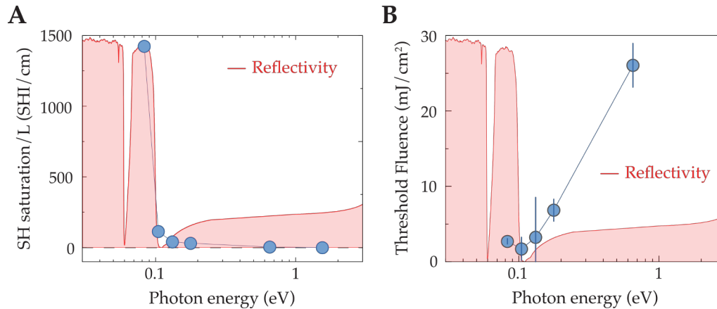
Figure 3.16: (A) saturation second harmonic intensity (parameter \alpha ) divided by the pump penetration depth. (B) Pump photon energy dependence of the threshold fluence (parameter \beta ).
