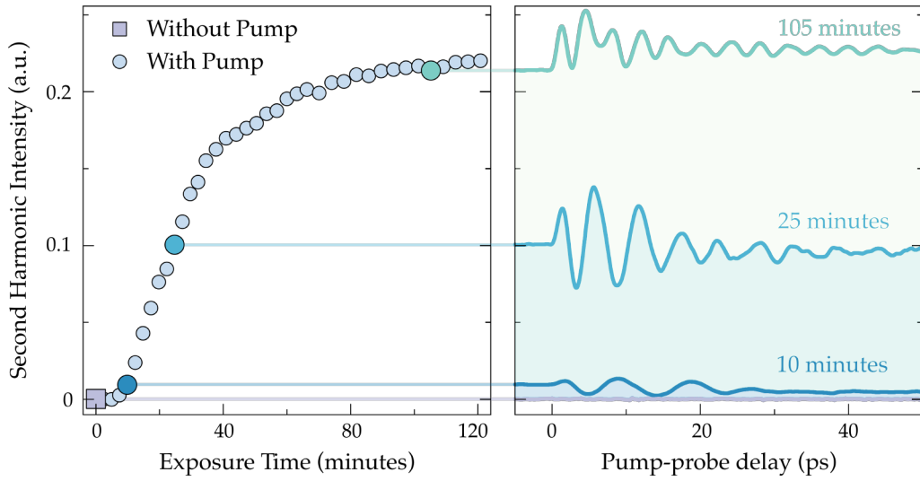
Figure 3.8: Light-induced symmetry breaking. Left: growth of baseline second harmonic signal as a function of exposure time to mid-infrared radiation. Note that this signal is independent on the pump-probe delay. Right: ultrafast pump-induced dynamics.
