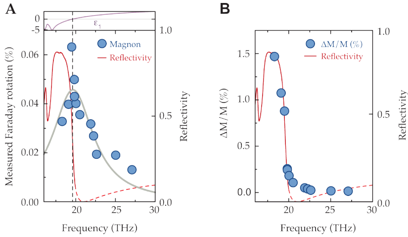
Figure 4.10: Wavelength dependence. (A) magnon amplitude as a function of pump wavelength (dots). The data is compared to the static reflectivity (red line) and real part of the dielectric function of the material (purple line). The dotted black line highlights the zero-crossing of the real part of the dielectric function. The grey line constitutes a guide to the eye. All measurements were taken at a constant fluence of 20 \frac{mJ}{cm^2} . (B) Retrieved total magnetization change. The pump-probe penetration-depth mismatch was taken into account to estimate the absolute change of magnetization.
