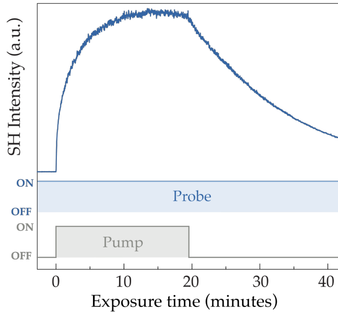
Figure 3.12: Polar state stability under continuous sampling. The mid-infrared light was only active for the first ~20 minutes of the experiment while the probe sampled the second harmonic continuously.
