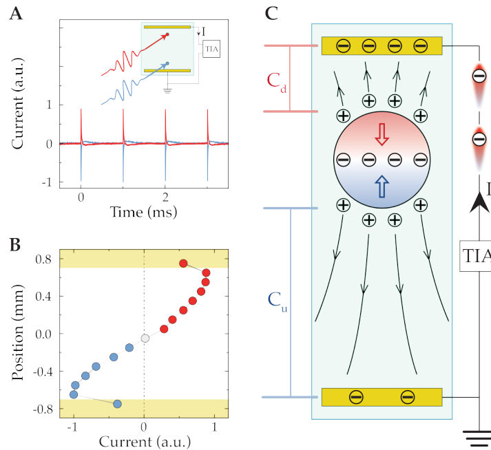
Figure 3.24: Spatial dependence of the electrical response. (A) Current pulses with different amplitudes and polarities were detected for the pump impinging closer to one of the two contacts. (B) Current pulses peak amplitude as a function of the pump position with respect to the contacts (yellow). (C) Schematic explanation of the detected current distribution. The domains position relative to the contacts determines the current amplitude and sign.
