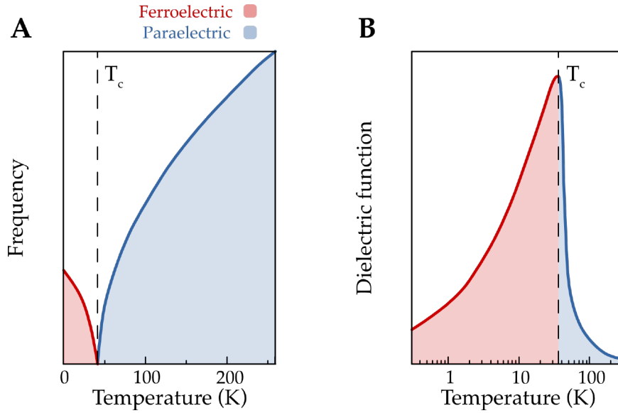
Figure 3.1: Fingerprints of a ferroelectric transition. (A) complete softening of the lowest energy polar phonon. (B) divergence of the dielectric function at the transition temperature.
