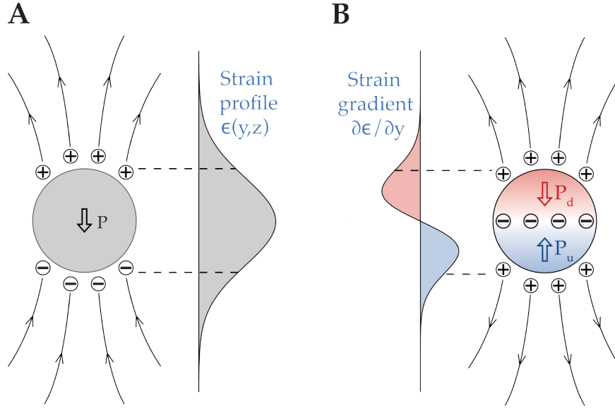
Figure 3.20: Possible domain profiles. (A) Strain profile that follows the Gaussian shape of the pump intensity. A direct, strain-induced transition results in a ferroelectric monodomain. (B) Inhomogeneous strain leads to the formation of two distinct flexoelectric domains, characterized by opposite polarities. In this case, the polarization profile follows the strain gradient.
