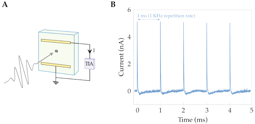
Figure 3.18: Light-driven current pulses. (A) Transport measurements setup. The photo-induced electrical response was measured in short-circuit conditions without applying any bias. Two gold electrodes were deposited on the sample surface, one connected to ground and the other to a transimpedance amplifier (TIA) which shares the same ground. (B) Electrical currents induced in unbiased SrTiO_3 by successive pump pulses (1-kHz repetition rate).
