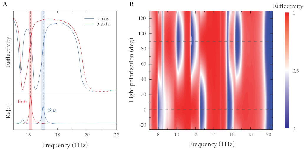
Figure 4.2: ErFeO_3 reflectivity. (A) Top: reflectivity for light polarization along the a and b crystallographic axes in blue and red, respectively. Bottom: real part of the optical conductivity. The peaks identify the frequency of the TO phonon. (B) polarization dependent reflectivity.
