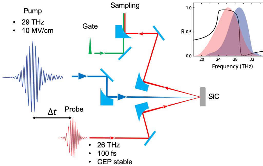
Figure A.4: Sketch of the experimental setup. The inset shows the spectral content of the pump (blue) and probe (red) pulses.
