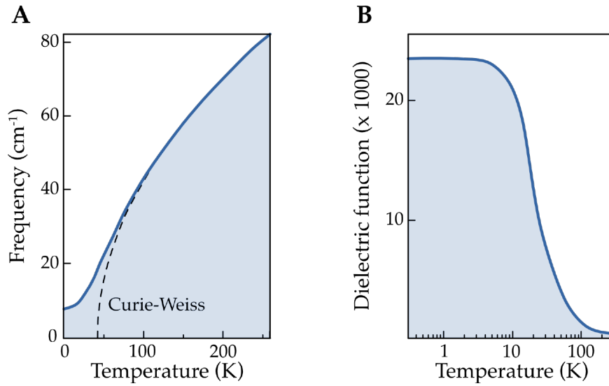
Figure 3.3: Incipient ferroelectricity in SrTiO_3 . (A) incomplete softening of the lowest energy polar mode (adapted from [106]). (B) despite a strong increase with decreasing temperatures, the dielectric function does not diverge (adapted from [133]).
