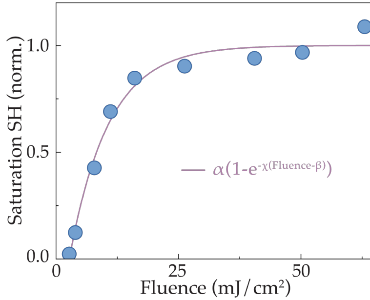
Figure 3.14: Pump fluence dependence. Second harmonic saturation value as a function of pump fluence. The pump wavelength was tuned to 15 \mu\text{m} . Note that in estimating the fluence values, because the pump power was measured outside the cryostat, the diamond window absorption was not considered.
