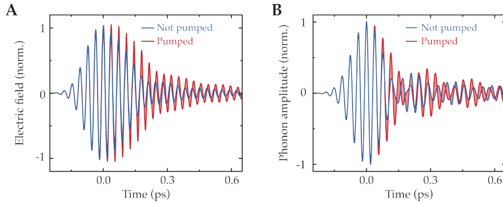
Figure A.7: Simulation results showing that to a pump-induced increase of the electric field reflected from the sample (A) corresponds an amplification of the phonon oscillations amplitude (B).
