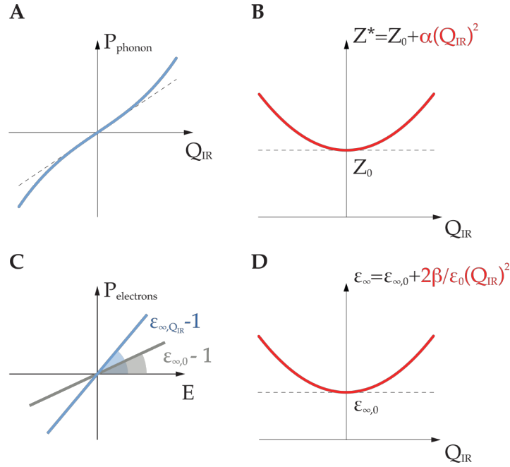
Figure A.1: Nonlinear expansion of the ionic and electronic contributions to the polarization in a solid, calculated from DFT. (A) Phonon polarization P_{phonon} . (B) Born effective charge. (C) Electronic polarization. The slope is given by the permittivity \epsilon_\infty which is shown in (D).
