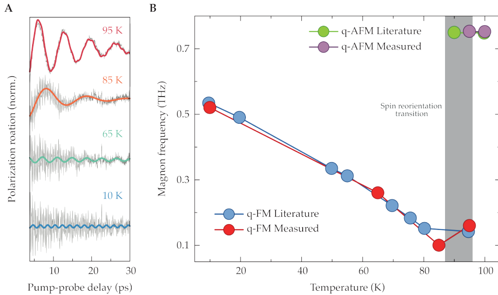
Figure 4.15: Temperature dependence of the magnetic oscillations. (A) Pump-induced polarization rotation at different sample temperatures. The signal comprising of both magnetic and vibrational excitations is shown in grey. The colored lines represent the magnon dynamics. The frequency of the oscillations changes dramatically with temperature. (B) Comparison of the detected frequency with literature data (from [131]). By changing the temperature of the system and, thus, the spin orientation, different magnon branches can be selectively excited.
