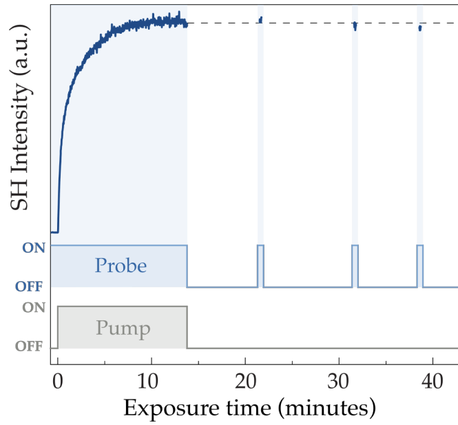
Figure 3.10: Polar state stability. The remaining second harmonic intensity was rarely and briefly sampled after removal of the pump.
