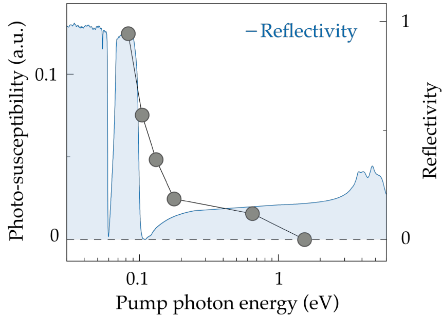
Figure 3.15: Wavelength dependence of the photosusceptibility. The equilibrium reflectivity of SrTiO_3 is shown in light blue.
