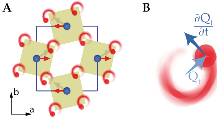
Figure 4.11: Circularly polarized phonons. Due to the non-degenerate nature of the driven vibrational modes, the ionic motion results in an elliptically polarized phononic field.
