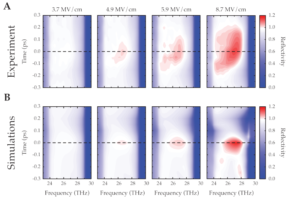
Figure A.6: Time and frequency dependent reflectivity for different intensities of the driving field. (A) Experimental results. (B) Simulations.
