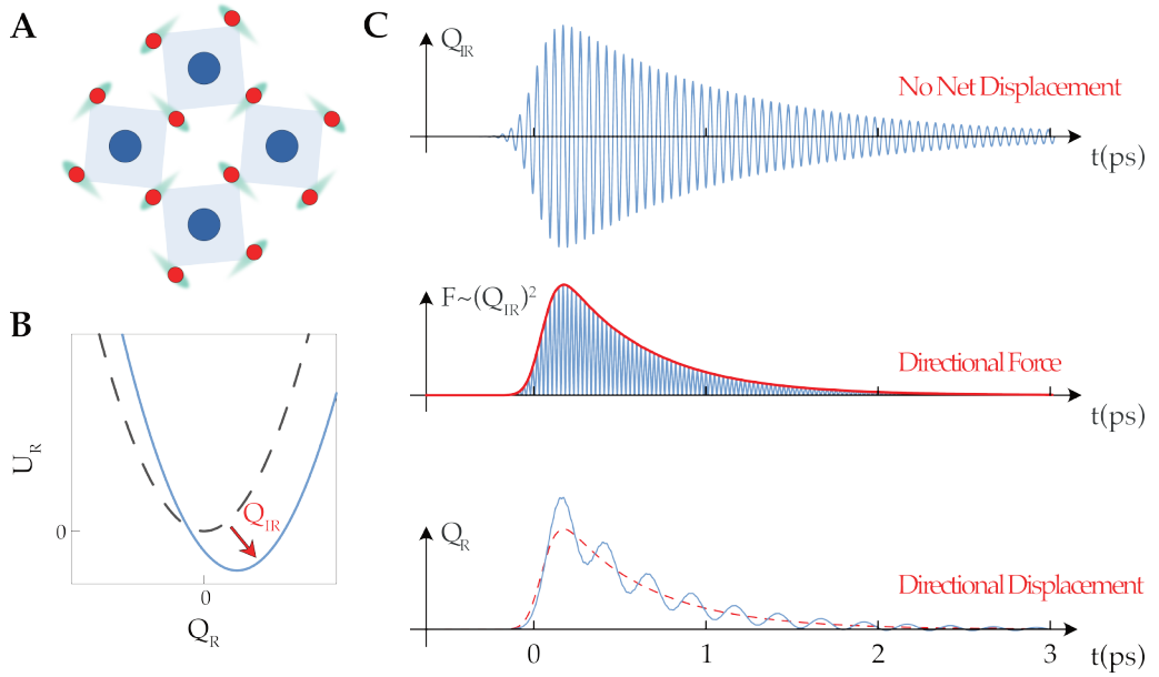
Figure 2.5: Nonlinear phononics. (A) representative Raman mode eigenvector in an insulating oxide. The mode does not possess a dipole. (B) harmonic potential for the Raman phonon. For finite amplitudes of the infrared phonon, the potential of the Raman mode is shifted towards a new equilibrium position. (C): Simulated nonlinear phonon dynamics. A 150 fs laser pulse drives resonantly a 20 THz infrared active phonons. The nonlinearly coupled Raman mode has a 4 THz resonance frequency. Top Panel: time-dependence of the displacement vector of a coherently driven phonon. Middle Panel: time-dependence of the force acting on the ions along the Raman coordinate. Bottom Panel: time evolution of the inelastically coupled Raman mode. Fig. B and C are inspired by [75].
