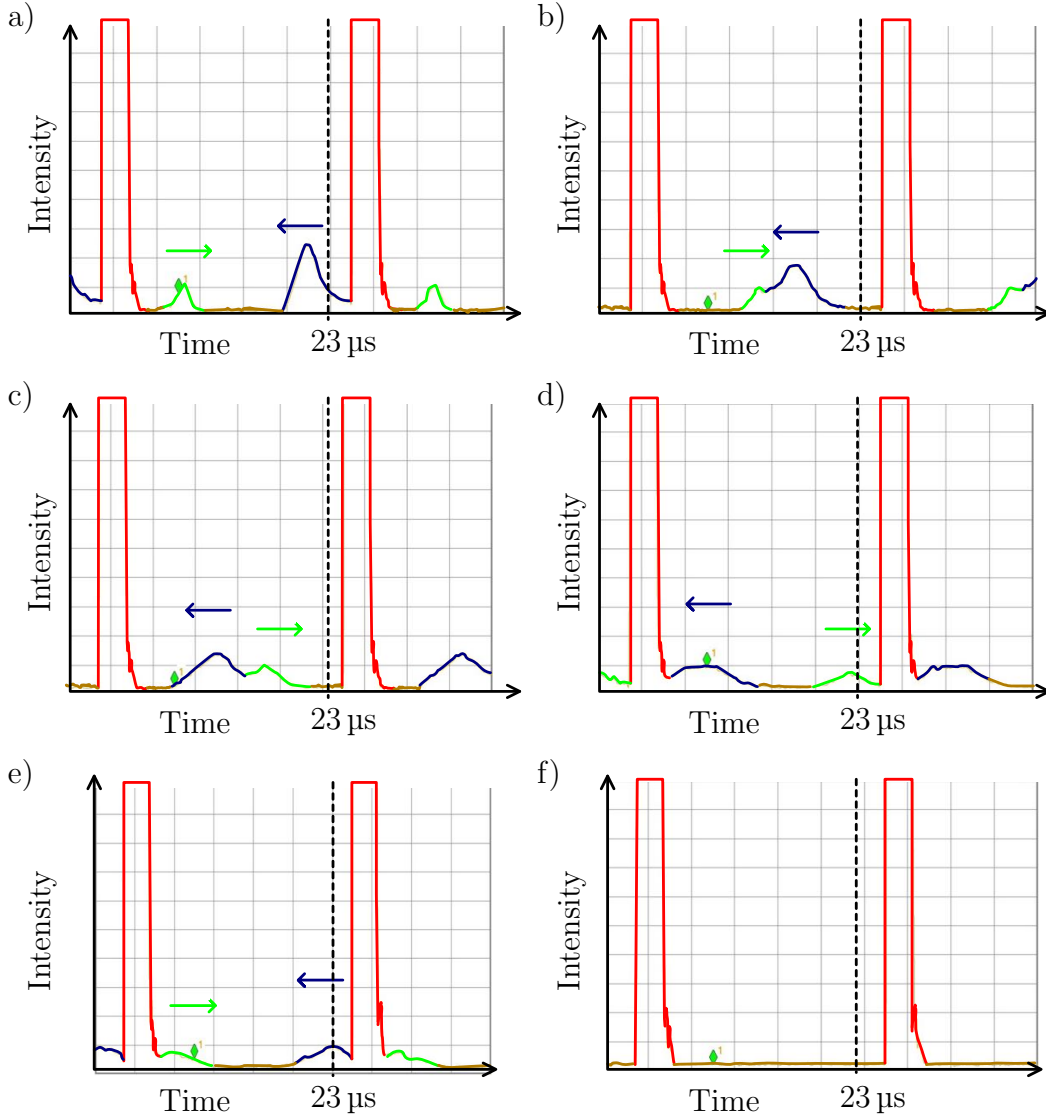
Figure 42: Measurements of the beam intensity in the SPS at different times of the injection plateau a) - e). The revolution period is about 23\ \mu\text{s} , one and a half turns of the SPS are displayed. The very high signal (red) originates from the train of the nominal bunches. The two much lower signals correspond to the un-captured particles coasting along the SPS. The distribution of particle with higher energy E > E_0 , green, have a longer orbit thus they move from left to right. The particles with lower energy E < E_0 , blue, move from right to left, they have a shorter orbit. The dispersion of the un-captured particles leads to a broadening of the distributions. During the acceleration process the un-captured particles are lost. The re-captured particle intensities are so small that they can not be resolved with these measurements f).
