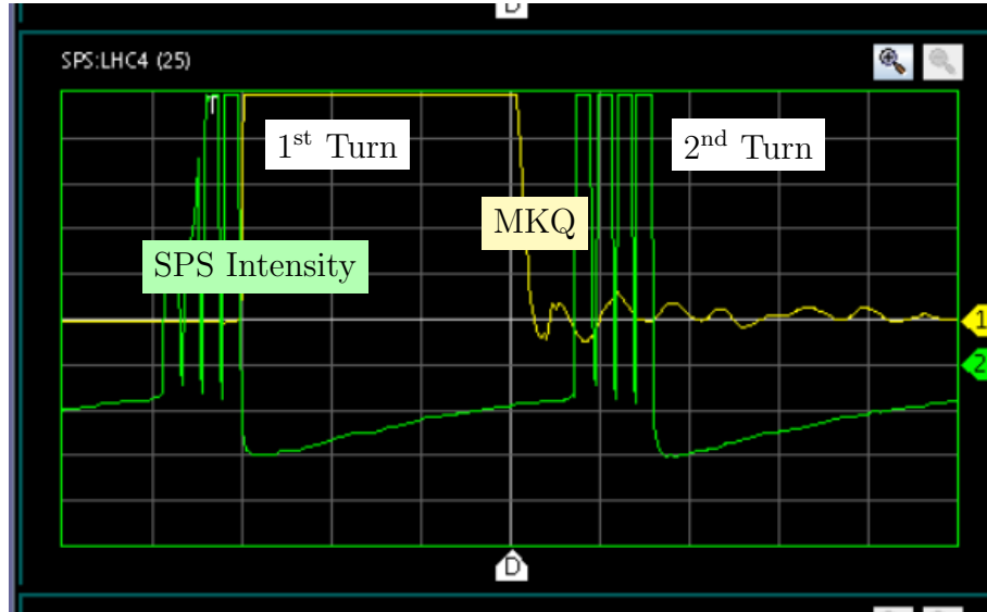
Figure 55: Screenshot of the SPS tune kicker display showing two turns of the SPS. The yellow line indicates the waveform of the MKQ's field. The green line represents the beam intensity in the SPS. The low bunch train signals in the first turn are electronics related. The beam intensity is constant. The four high signals result from the four trains of 72 bunches circulating in the SPS.
