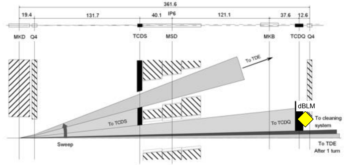
Figure 61: Conceptual layout of the LHC beam extraction in IR 6. The beam is steered by the extraction kicker magnets (MKDs) into the dump line towards the dump block (TDE). Absorber blocks (TCDS, TCDQ) protect the downstream accelerator components from mis-steered particles [58]. The diamond based beam loss monitor, yellow, downstream of the TCDQ detects the ultra fast extraction losses.
