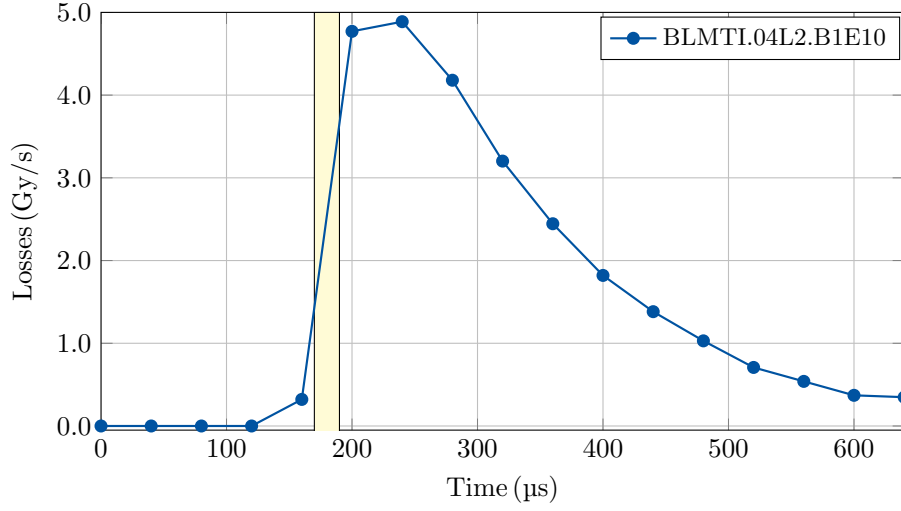
Figure 13: ultra fast injection loss signal recorded by the beam loss monitoring system with the shortest integration window length of 40\text{ }\mu\text{s} . The losses occur in the time window indicated with a yellow bar. The signal length is dominated by the response time of the beam loss monitor and the data acquisition system, long fall time after the initial short signal.
