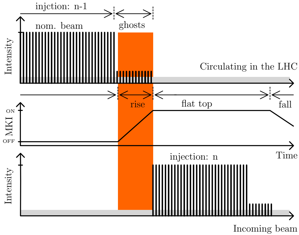
Figure 45: Creation of loss signal with ghost bunch structure. The trailing ghost bunches of the previous injection ( n-1 ) are deflected by the rising fields of the injection kicker magnets for the next injection ( n ). The deflected particles impact on the absorber block downstream of the injection kicker magnets, the TDI. The dBLM installed downstream of the TDI detects the secondary shower particles.
