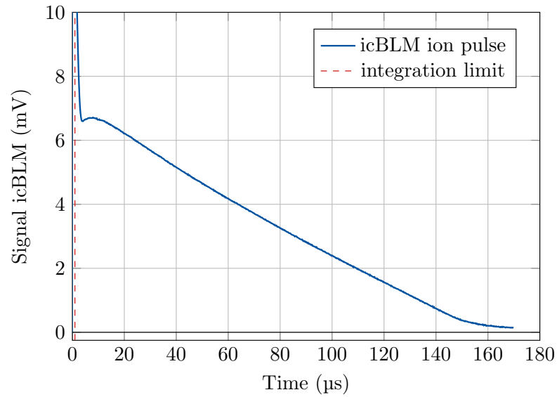
Figure 24: Averaged ion pulse shape of the icBLM. Compared to the electron pulse the signal created by the ions is much longer, about 170\,\mu\text{s} . The amplitude is about 6.8\,\text{mV} . The integrals of the electron signal and the ion signal are the same.
