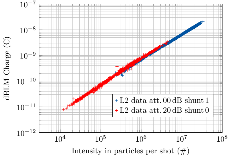
Figure 26: Response measurements of the detector L2. Two acquisition configurations were used. The signal was attenuated by 20 dB in the intensity regime below 4 \times 10^6 electrons/bunch. A 1- \Omega -shunt system was used for measurements in the intensity regime of more than 10^5 electrons/bunch. The measurements with both configurations overlap.
