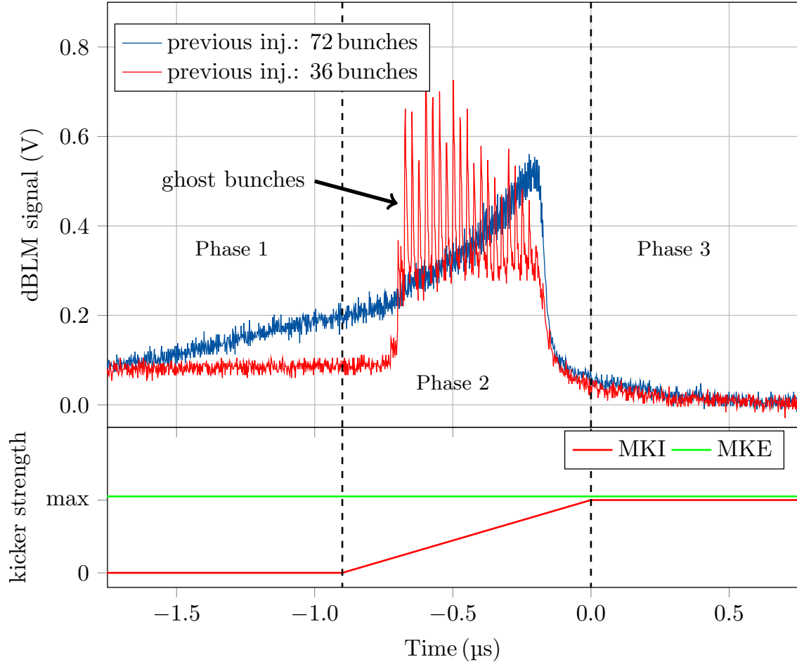
Figure 48: Injection losses of two injections with injected 144 bunches. For the injection, which is preceded by an injection of 72 bunches, blue, no ghost bunches were detected. In the loss signature of the injection, which was preceded by an injection of 36 bunches, red, the ghost bunches were clearly visible. The vertical lines separate the different phases of the injection loss signatures. In the plot below the status of the SPS extraction kicker and the LHC injection kickers are displayed.
