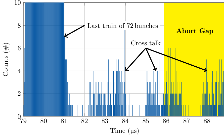
Figure 67: Zoom into the end of the filling pattern of the loss histogram shown in Fig. 66. In this case the gap was longer as the indicated 3\mu\text{s} due to a reduced number of bunches in the beam. The cross talk from the second beam is visible. The data is smeared out so that single bunches can not be identified.
