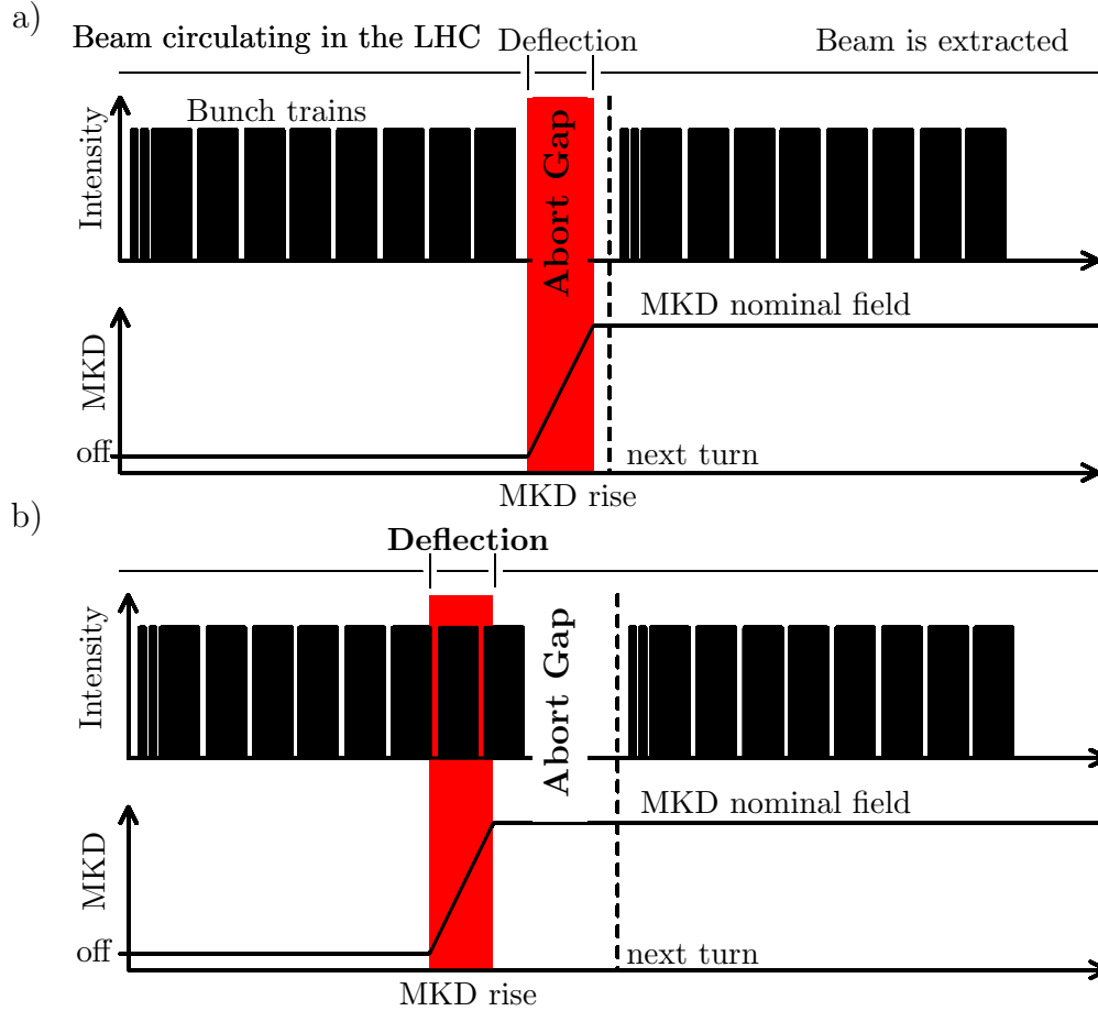
Figure 63: The extraction kicker magnets (MKD) have a rise time of about 2.9\mu\text{s} , red. During a normal dump procedure, a), the extraction kickers are synchronised to the 3\mu\text{s} long abort gap, so that ideally no high energetic particles are mis-steered due to rising kicker fields. The extraction kickers are at their nominal field strength when the next bunches pass, so that the beam is steered into the extraction line and safely dumped. In case of an asynchronous beam dump, b), the extraction kicker magnets are triggered without the synchronisation to the abort gap. In this case high intensity bunches are deflected by the rising kicker fields, which results in massive beam losses in the extraction region leading to quenches in the downstream magnets.
