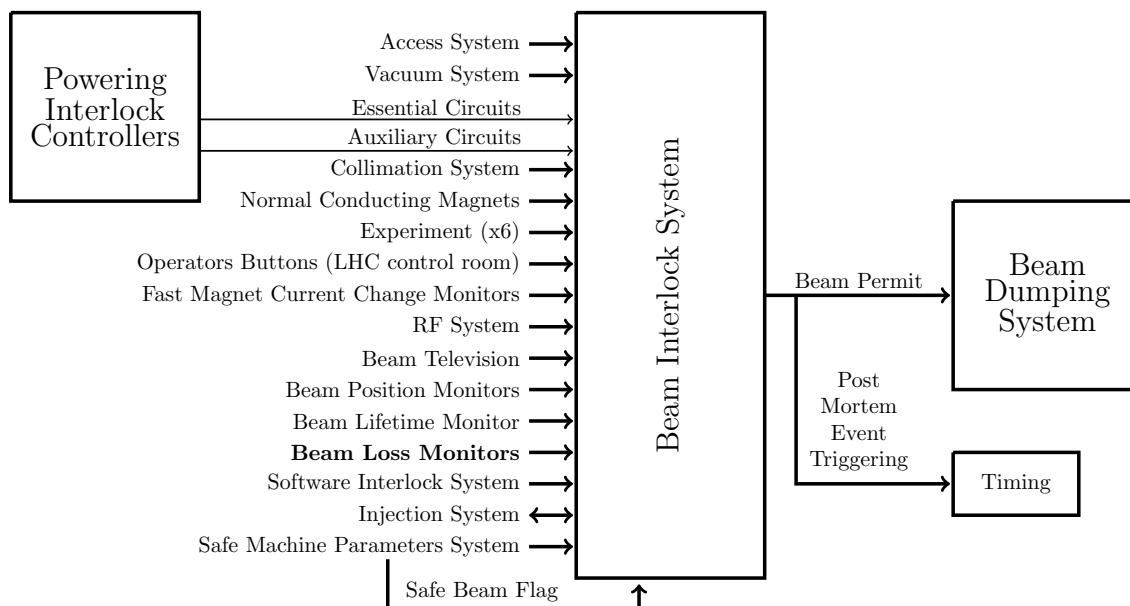
Figure 11: The beam interlock system gets input from various subsystems. If one of the subsystems raises an error the beam permit is cancelled and the beams are dumped [18].
