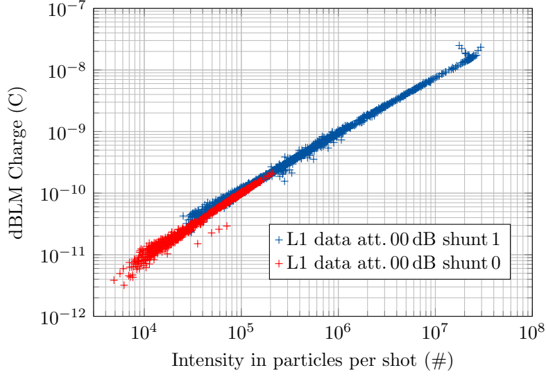
Figure 25: Response measurements of the detector L1. Two acquisition configurations were used. No shunt or signal attenuation in the intensity regime of less than 10^5 electrons/bunch. A 1- \Omega -shunt system was used for measurements in the intensity regime of more than 10^5 electrons/bunch. The measurements with both configurations overlap.
