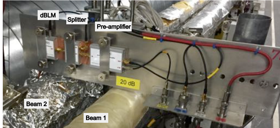
Figure 30: Frontend electronics of the LHC type dB LM as it is installed in IR 7 beam 2. The dB LM is installed centred above the beam pipe of beam 2. The signal AC signal is split from the DC component by a splitter. The adjacent pre-amplifier amplifies the signal by 20 dB.
