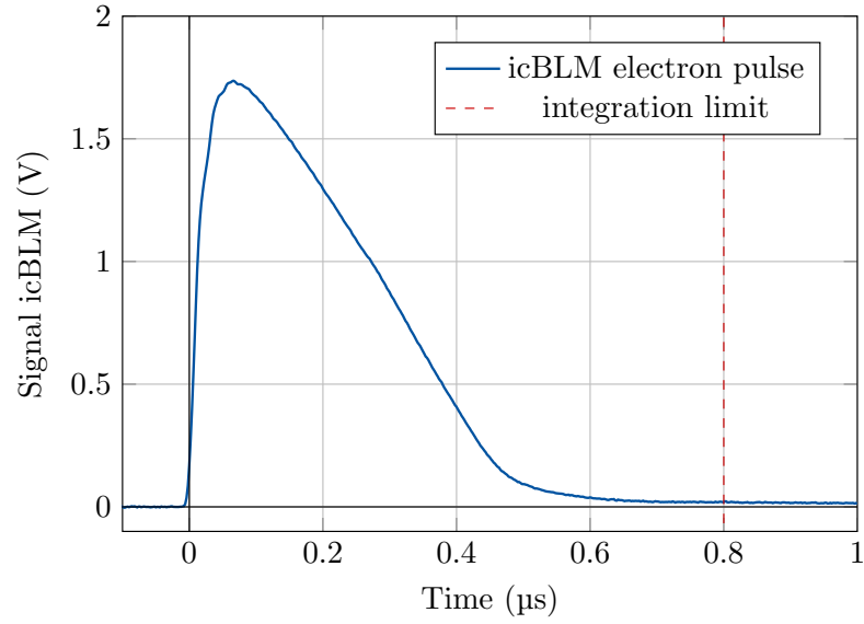
Figure 23: Averaged electron pulse shape of the icBLM. The signal created by the much more mobile electrons is about 0.8\,\mu\text{s} long and has an amplitude of 1.7\,\text{V} , which is much higher than the ion pulse.
