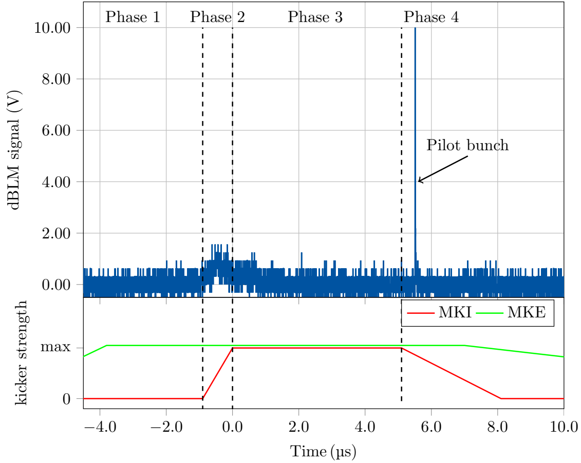
Figure 60: Over injection of a misplaced pilot bunch, same event as shown in Fig. 59, recorded on the low gain channel of the readout electronics which covers a larger range of loss amplitudes. The pilot loss signal amplitude exceeds the rest of the loss signature by two orders of magnitude which makes this loss signal even more visible and easy to identify.
