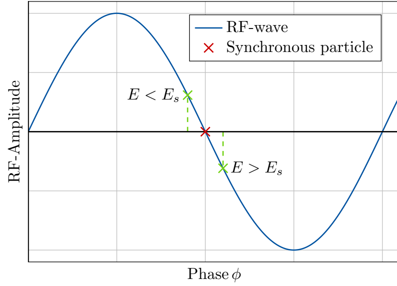
Figure 5: Phase of the synchronous particle with out acceleration. The synchrotron motion of the off-momentum particles keep the beam bunched.
