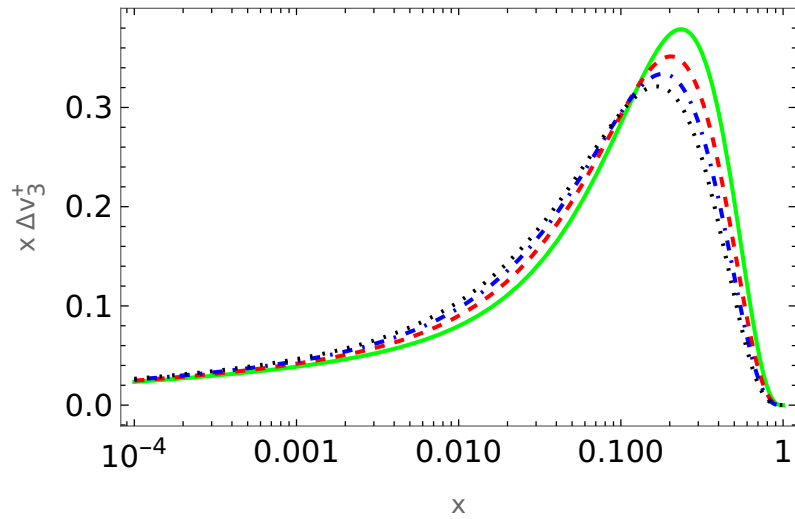
Figure 25: The polarized PDF \Delta v_3^+(x, Q^2) resulting from the LO evolution of the input (8.164). Solid lines: Q^2 = 10 \text{ GeV}^2 . Dashed lines: Q^2 = 10^2 \text{ GeV}^2 , Dash-dotted lines: Q^2 = 10^3 \text{ GeV}^2 ; Dotted lines: Q^2 = 10^4 \text{ GeV}^2 .
