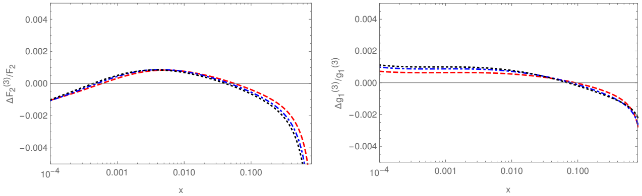
Figure 12: The effect of the variation of P_{qq}^{3,\pm,\text{NS}} around the value in Eq. (5.28) by \pm 100\% . Dashed lines: Q^2 = 100 \text{ GeV}^2 , Dash-dotted lines: Q^2 = 1000 \text{ GeV}^2 ; Dotted lines: Q^2 = 10000 \text{ GeV}^2 . Left: F_2^{\text{NS}} ; Right: xg_1^{\text{NS}} .
