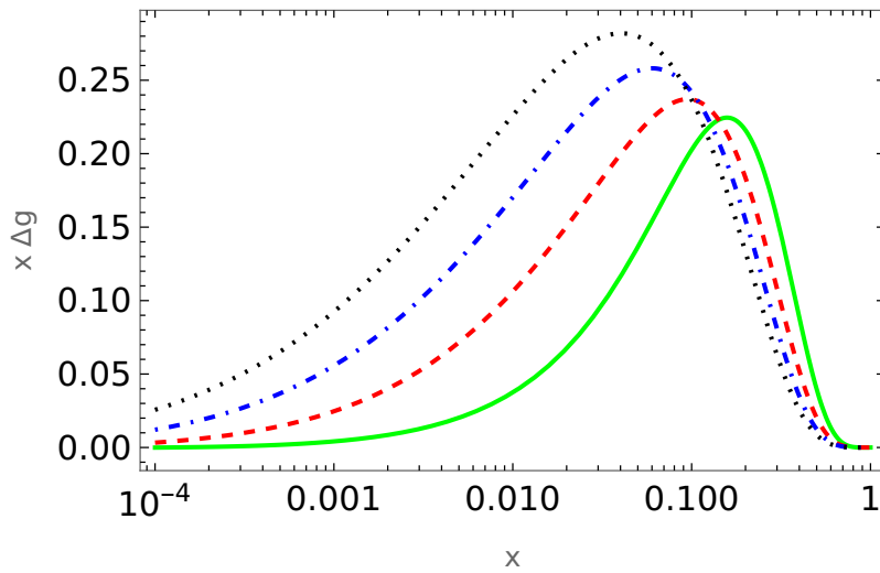
Figure 28: The polarized PDF \Delta g(x, Q^2) resulting from the LO evolution of the input (8.164). Solid lines: Q^2 = 10 \text{ GeV}^2 . Dashed lines: Q^2 = 10^2 \text{ GeV}^2 , Dash-dotted lines: Q^2 = 10^3 \text{ GeV}^2 ; Dotted lines: Q^2 = 10^4 \text{ GeV}^2 .
